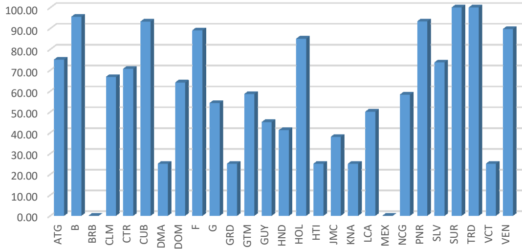
Iteration 36 - Percentage of assignable channels (1.25dB margin), ignoring self-interference and interference to the wanted requirement
