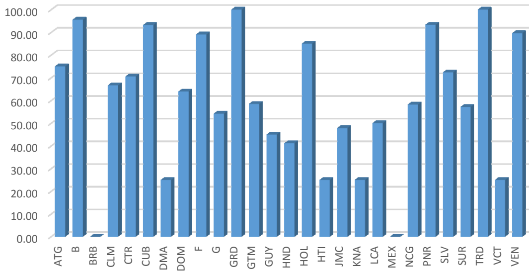
Iteration 33- Percentage of assignable channels (1.25dB margin)
