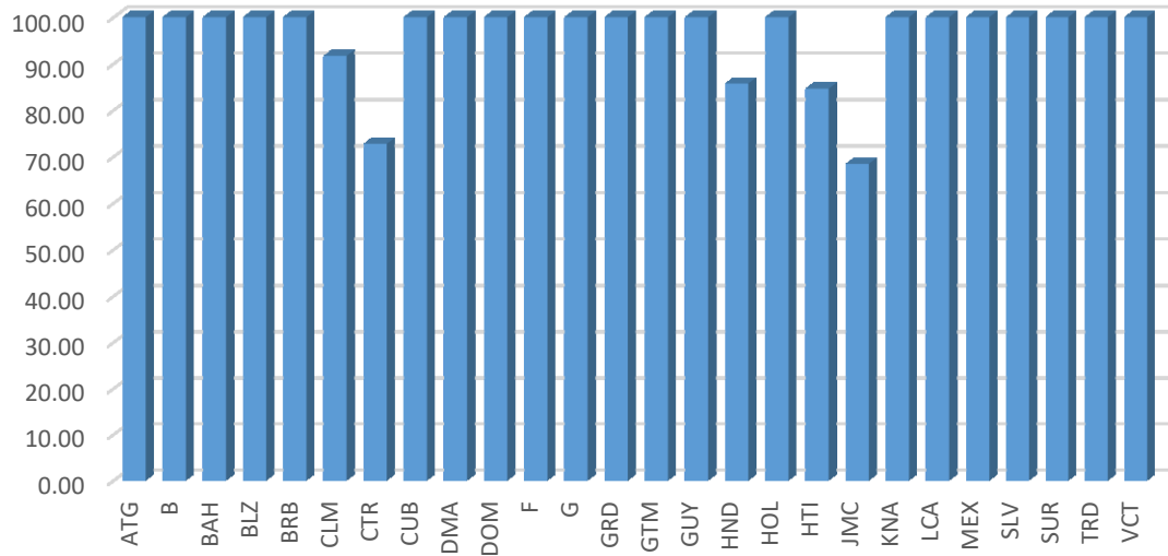
Final VHF iteration - Percentage of assignable channels (4dB margin), ignoring self-interference and interference to the wanted requirement
