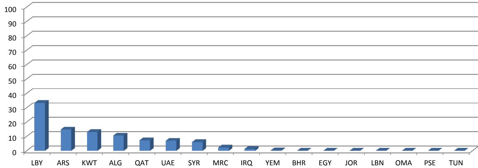
Iteration before Dubai meeting-Percentage of assignable channels with margin: 4dB
