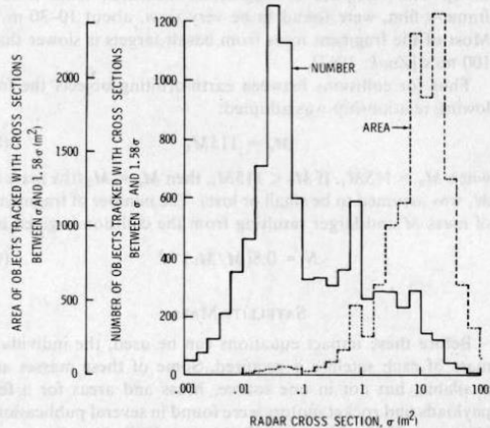
Fig. 3. Size distribution of earth-orbiting satellites observed by radar. The largest number of satellites have a radar cross section of about 0.04 m², while the largest area contribution is around a radar cross section of 10 m².
