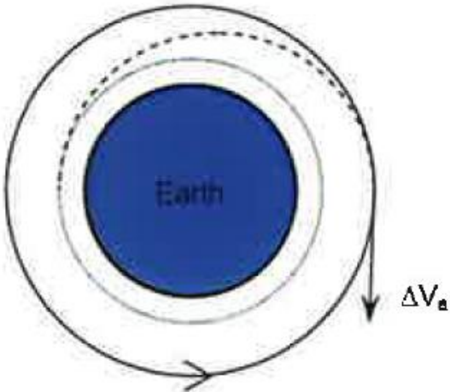
De-orbit procedure
