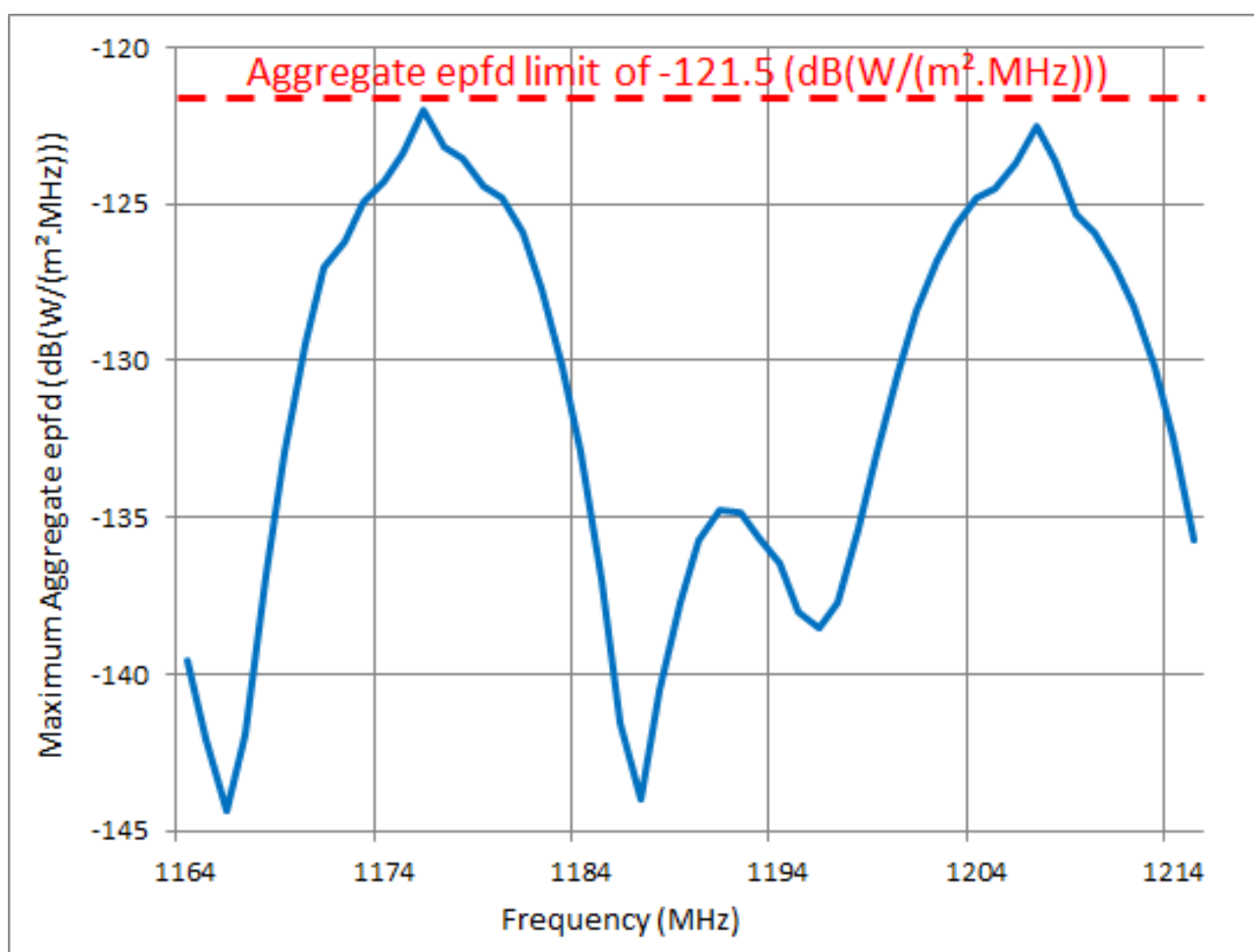
Figure 1: Plot of Table 2 (Maximum RNSS Aggregate epfd per MHz with 1° steps)
