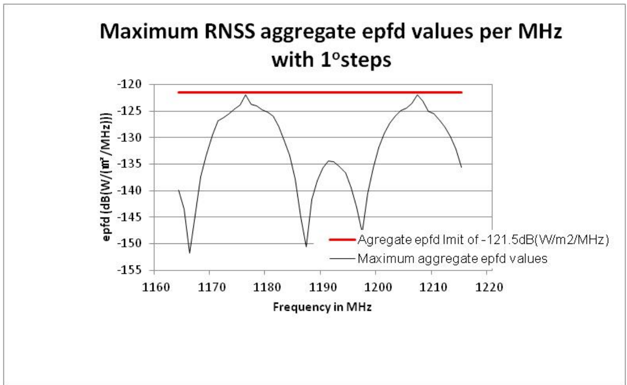
Figure 1: Plot of Table 2 (Maximum RNSS Aggregate epfd per MHz with 1° steps)
