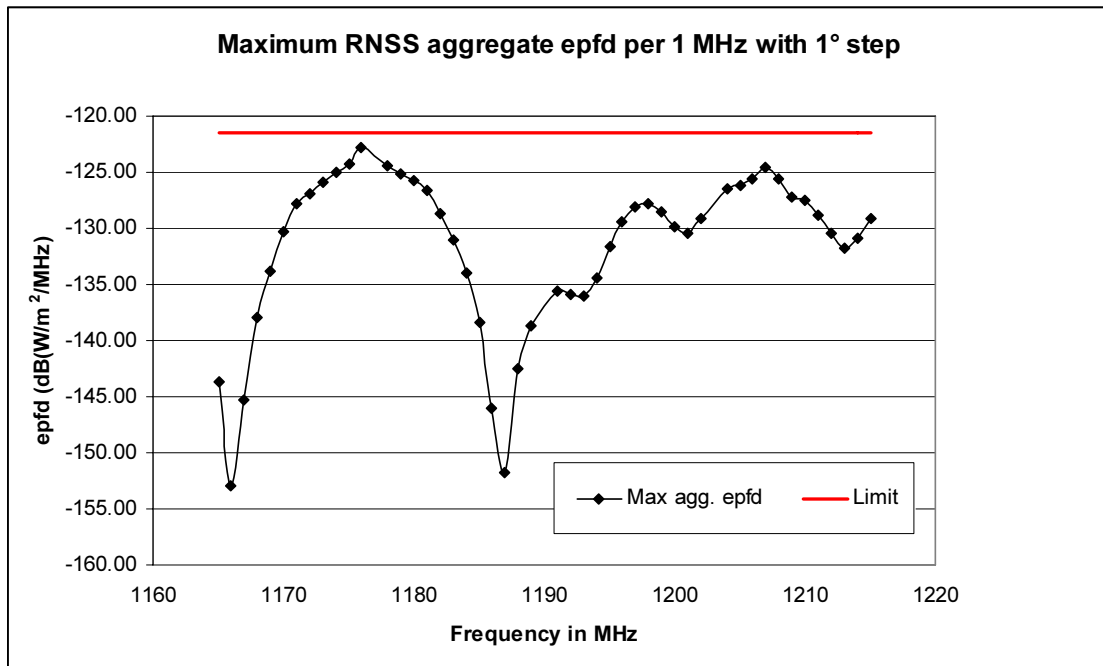
Figure 1: Plot of Table 2 (Maximum RNSS Aggregate epfd per MHz with 1° steps, without NIGCOMSAT-1G)
