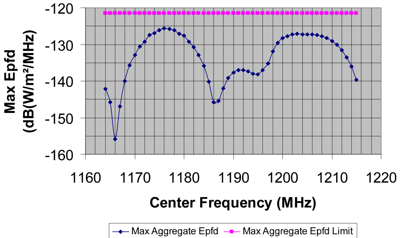
Figure 1: Plot of Table 2 (Maximum RNSS Aggregate epfd per MHz).
