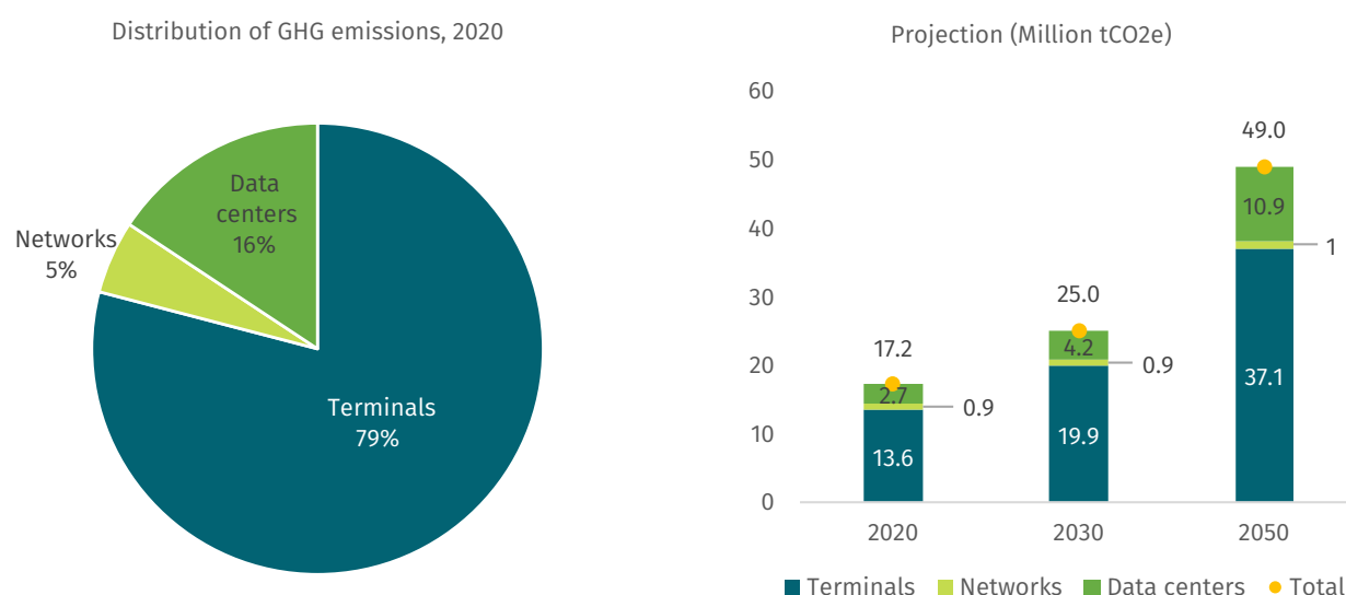
Figure 3.2: ICT carbon footprint in France
