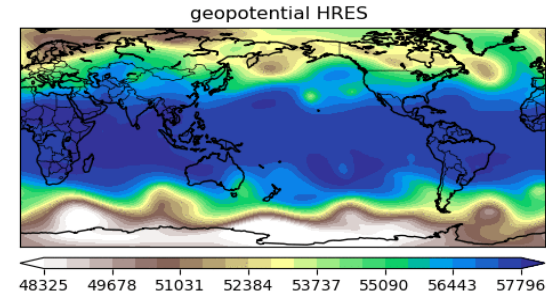
ECMWF Weather Model
