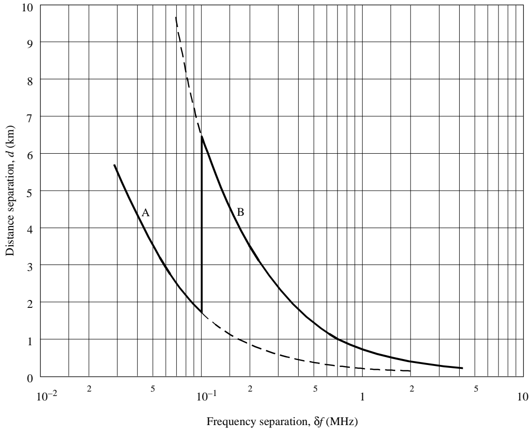
An FD rule for two-signal third-order receiver intermodulation interference analysis
