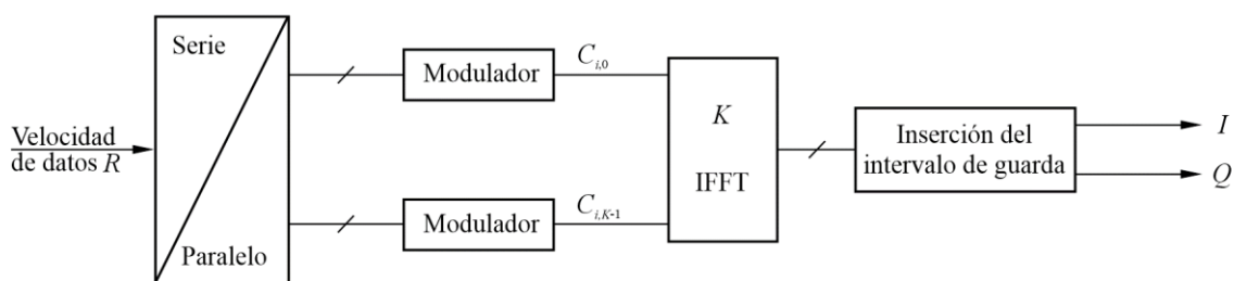
FIGURA 34 Transmisor MDFO
