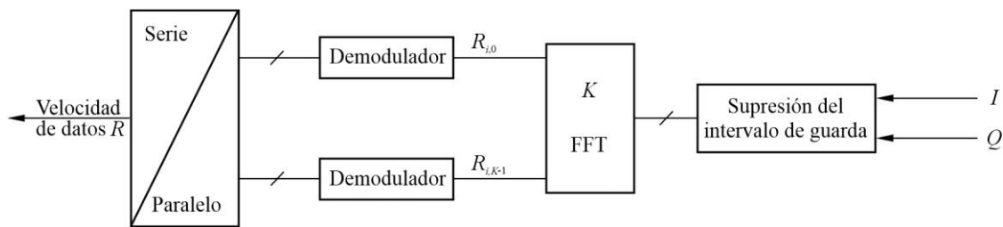
FIGURA 35 Receptor MDFO
