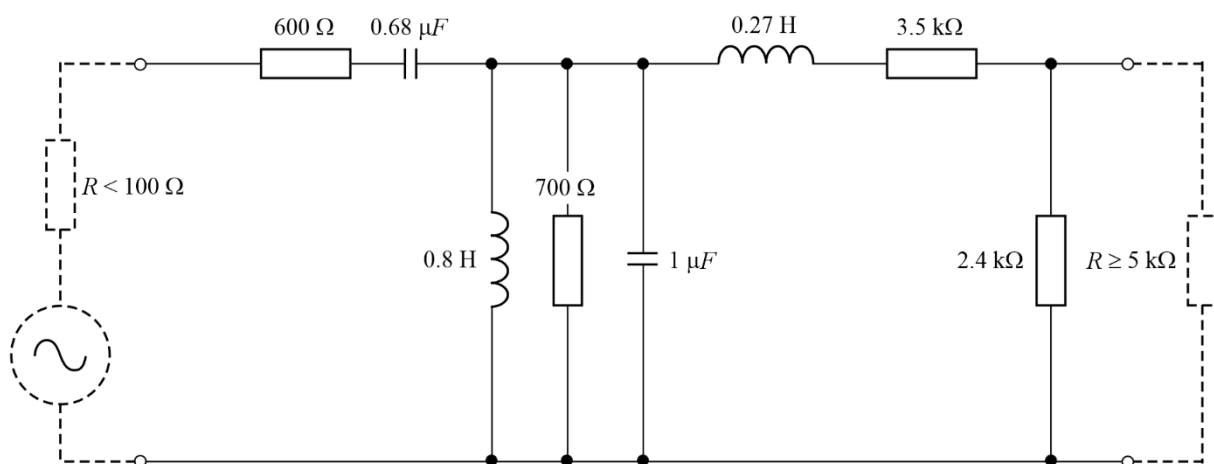
FIGURE 9 Filter circuit
