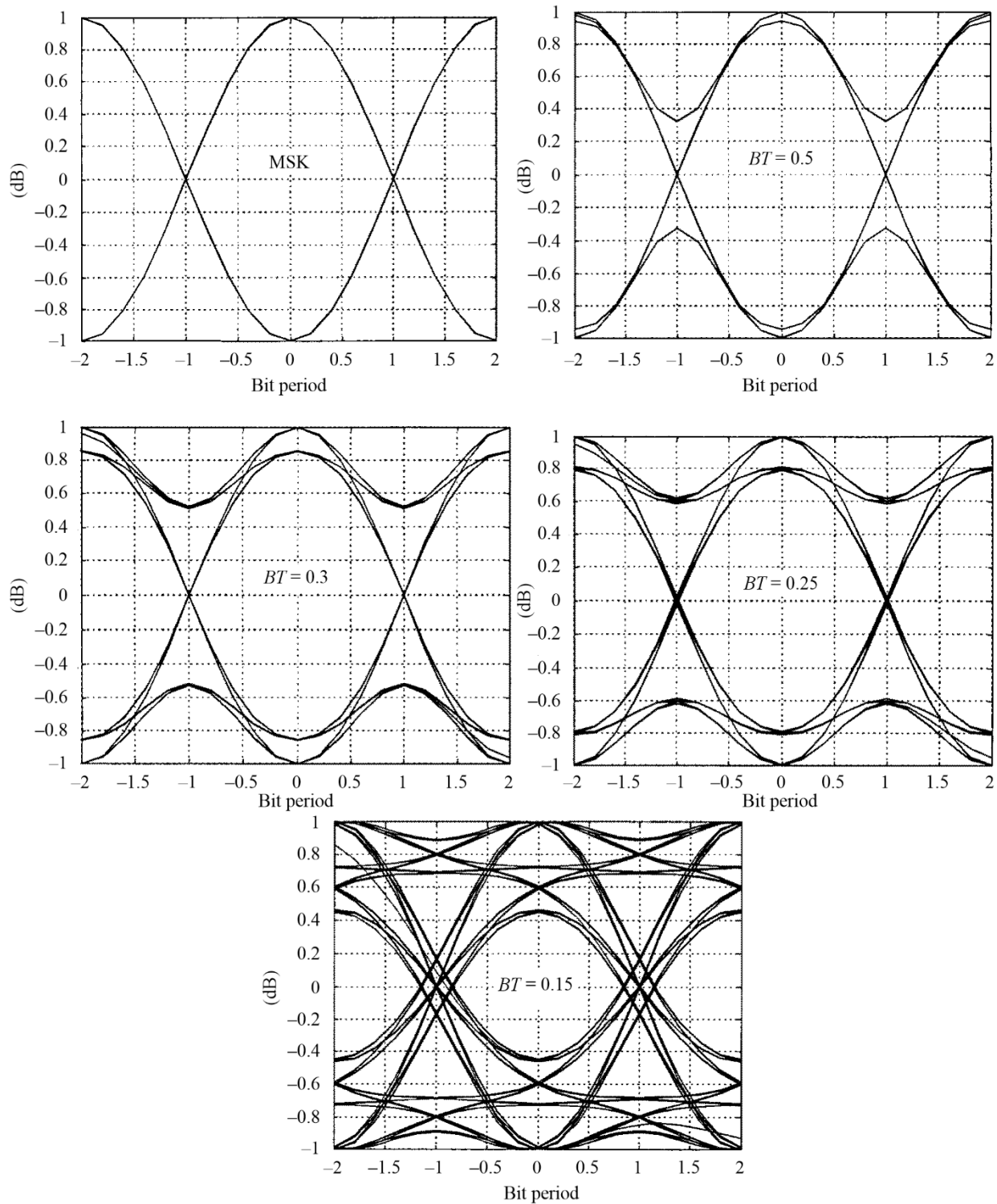
FIGURE 33 Eye diagrams
