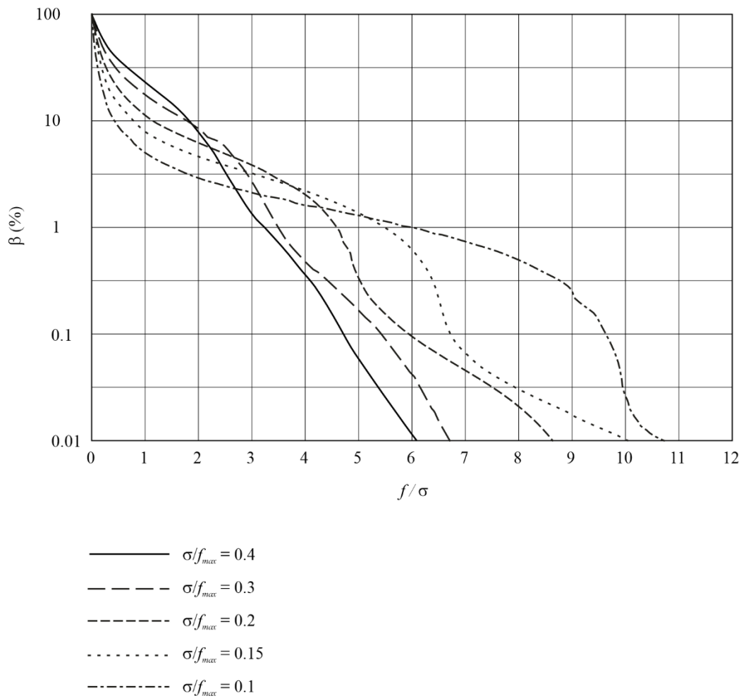
FIGURE 20 Out-of-band power of the spectra for \sigma / f_{max} < 0.5
