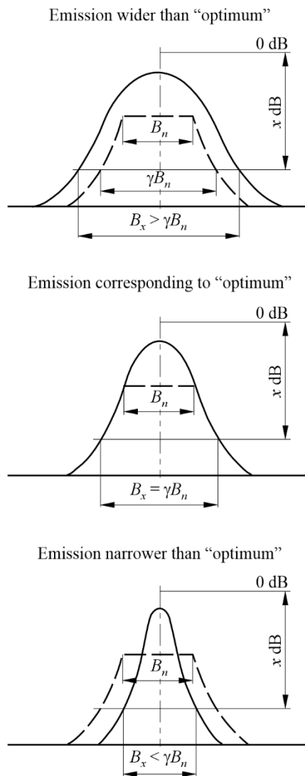
FIGURE 2 Evaluation of spectra, by means of the x dB bandwidth
