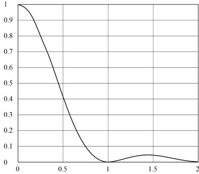
FIGURE 26 BPSK spectrum
