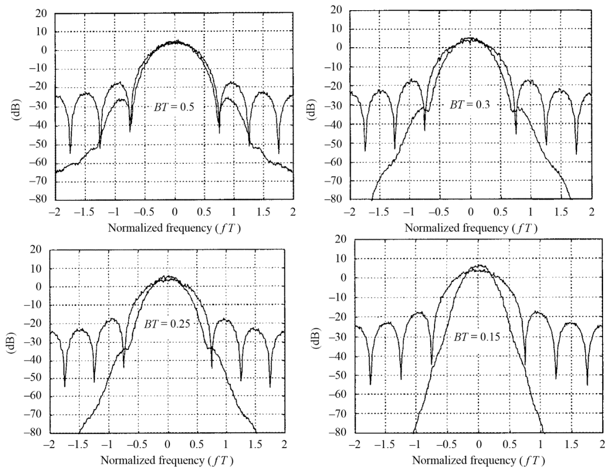
FIGURE 32 GMSK spectra for BT = 0.5, 0.3, 0.25 and 0.15
