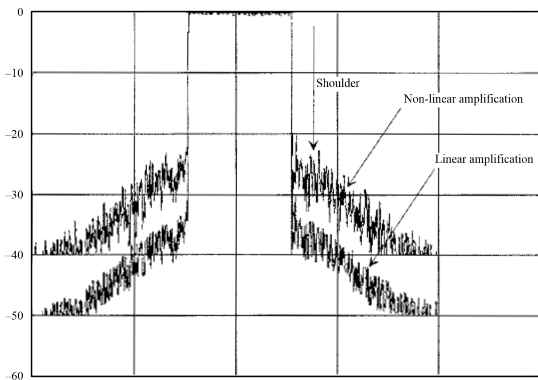
FIGURE 37 Linear and non-linear simulated OFDM spectrum
