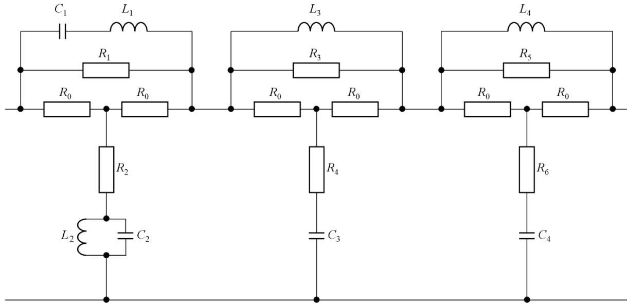
FIGURE 5 Shaping network of the conventional telephone signal generator
