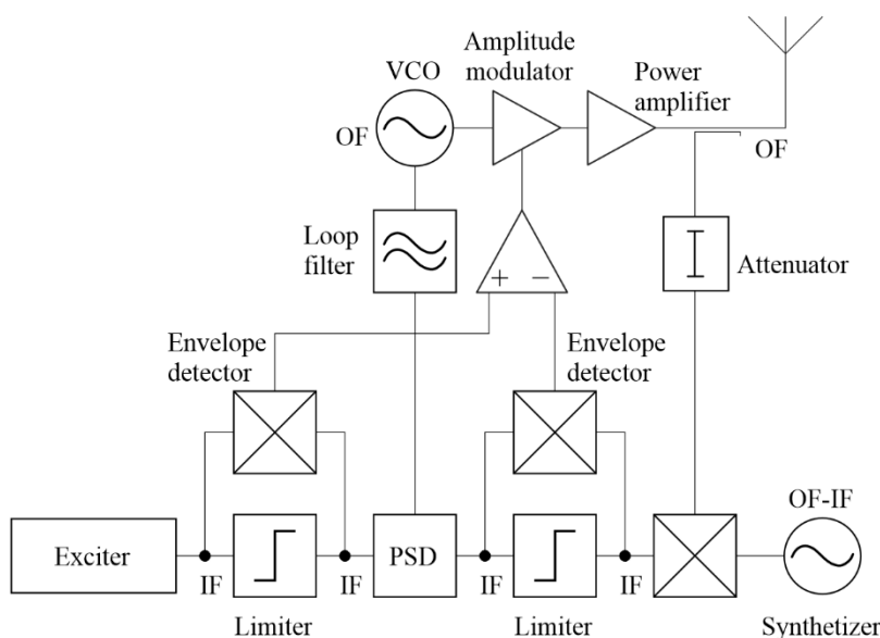
FIGURE 47 The Polar Loop technique
