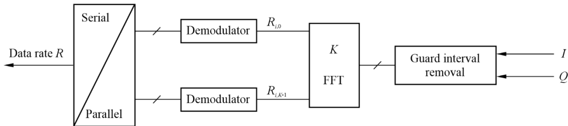
FIGURE 35 OFDM receiver
