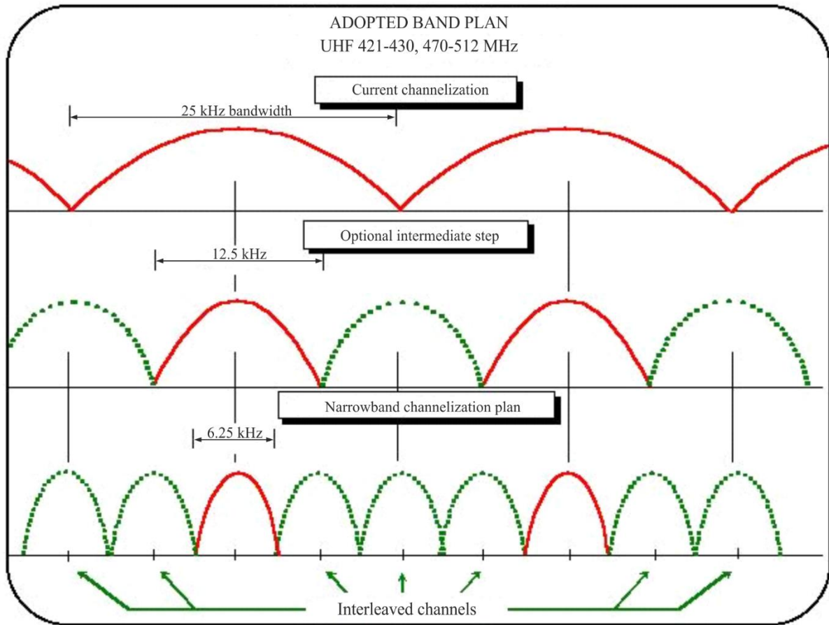
FIGURE 7 470-512 MHz Shared with UHF-TV; available only in 11 cities, channels are spaced every 6.25 kHz, authorized bandwidth is 20 kHz, 11.25 kHz or 6 kHz
