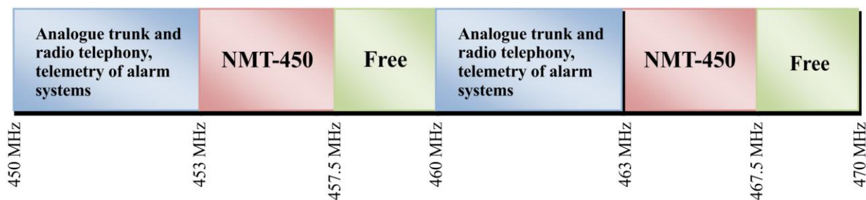
FIGURE 2 Frequency use in the band 450-470 MHz before redeployment
