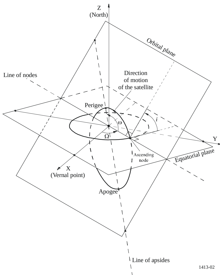
FIGURE 2 Non-geostationary orbital parameters
