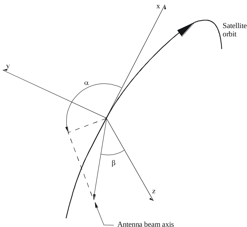
FIGURE 5 Orientation angles
