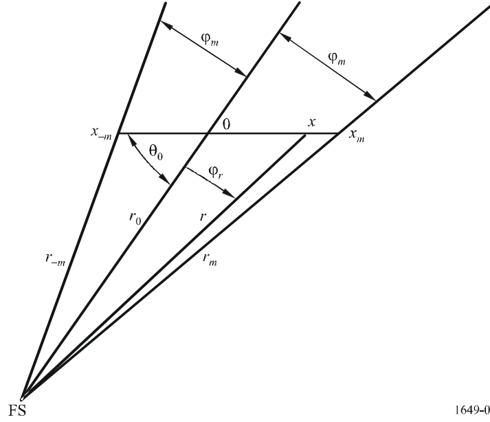
FIGURE 3 Geometry of a main beam passage of an ESV
