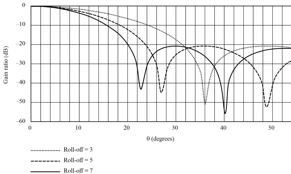
FIGURE 6 Radiation cutting of reference antenna diagram
