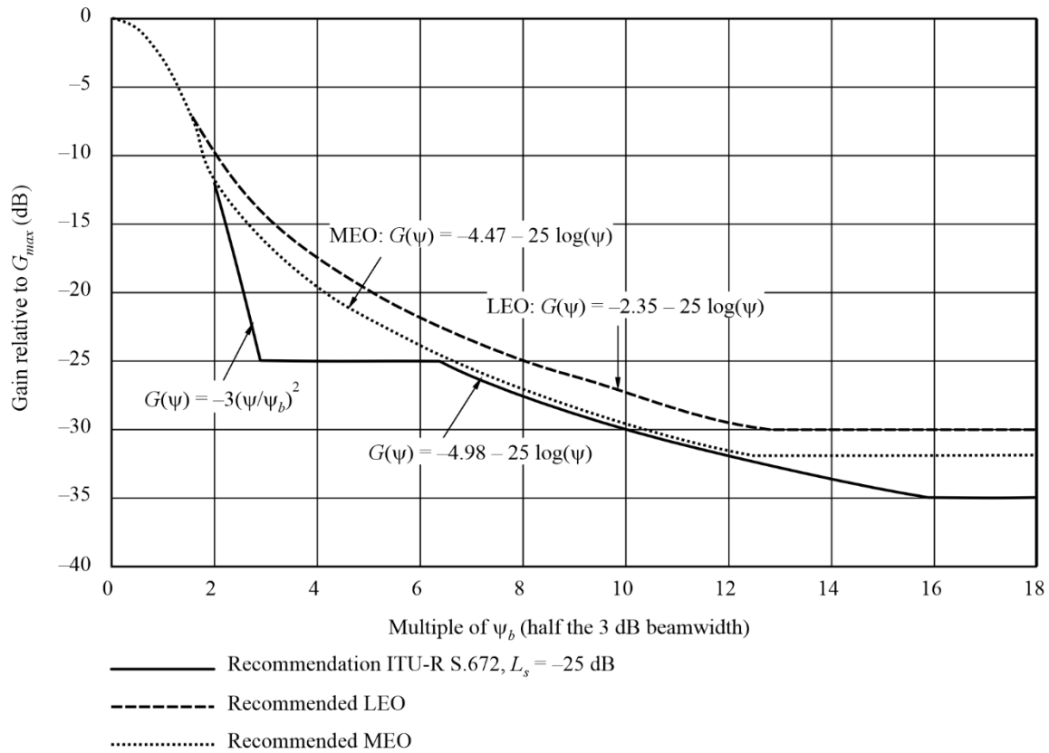
FIGURE 2 Reference radiation pattern for LEO, MEO and GSO
