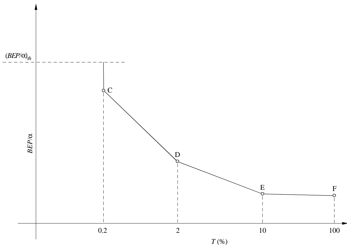
FIGURE 3 Simplified mask
