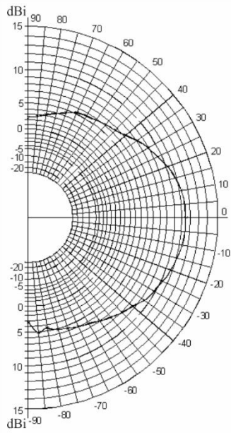
Radiation pattern (H-plane, 12 degrees angle) of antenna 2
