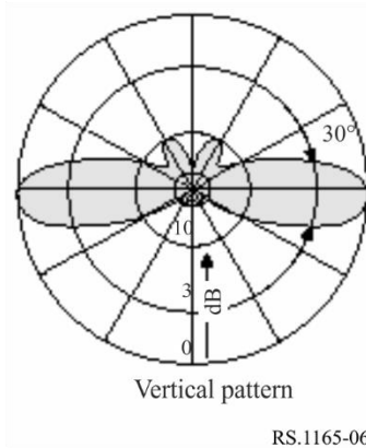
FIGURE 6 Radiation pattern of antenna 3
