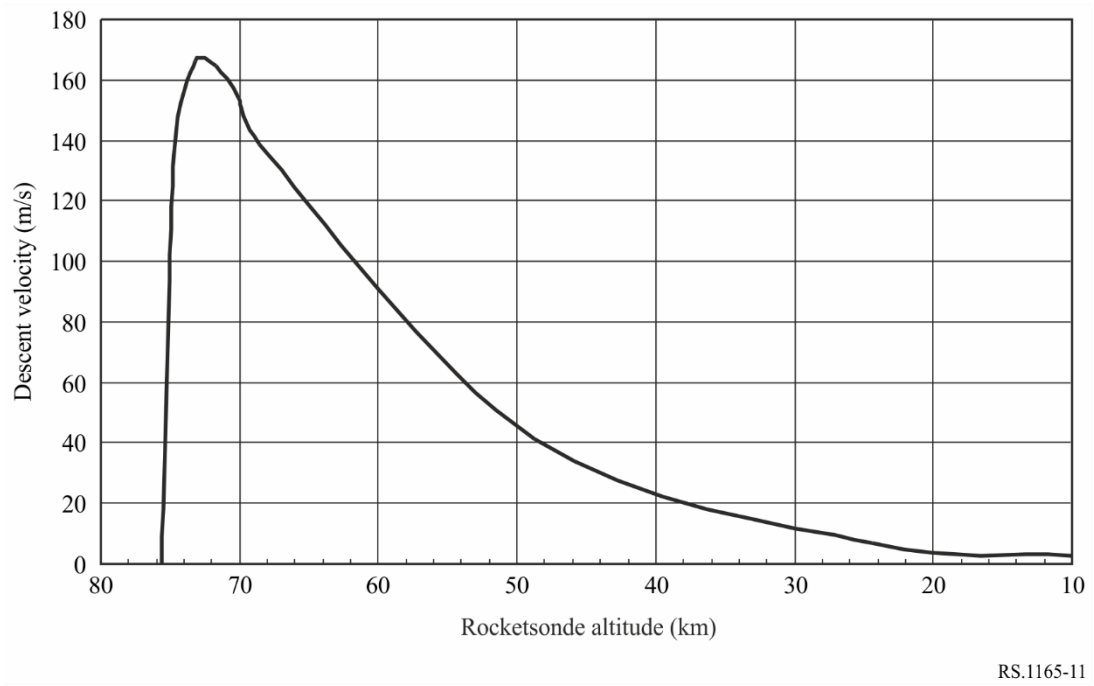
FIGURE 11 High altitude rocketsonde descent profile (altitude vs. descent velocity)
