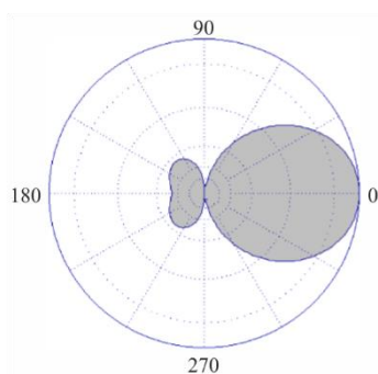
FIGURE 9 Radiation pattern of antenna 4
