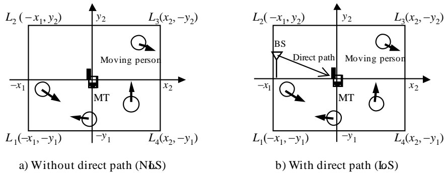
FIGURE 3 Rectangular-shaped room layout
