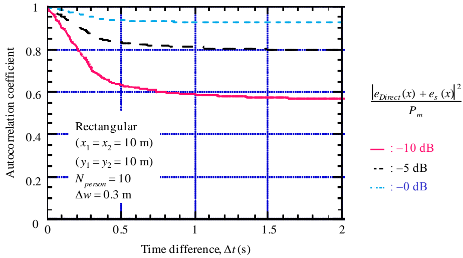
FIGURE 6 Autocorrelation coefficient of received level in circular room
