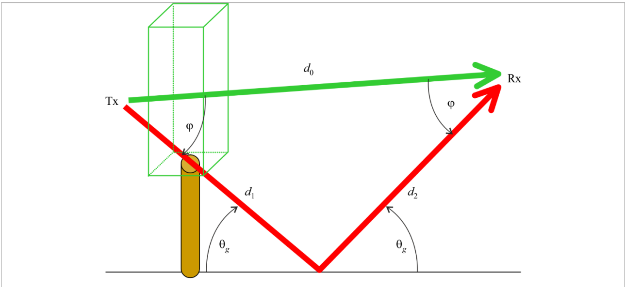
FIGURE 6 Ground reflected component
