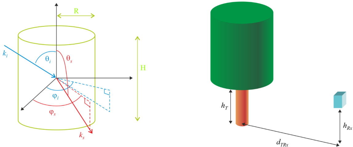
FIGURE 8 Geometry definition
