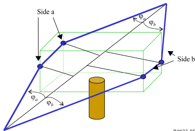
FIGURE 5 Components diffracted around the vegetation
