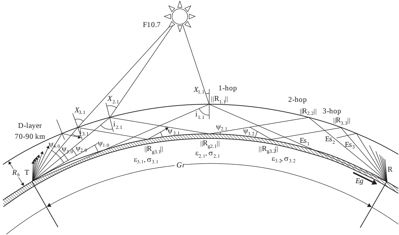
FIGURE 12 Propagation factors and path geometry
