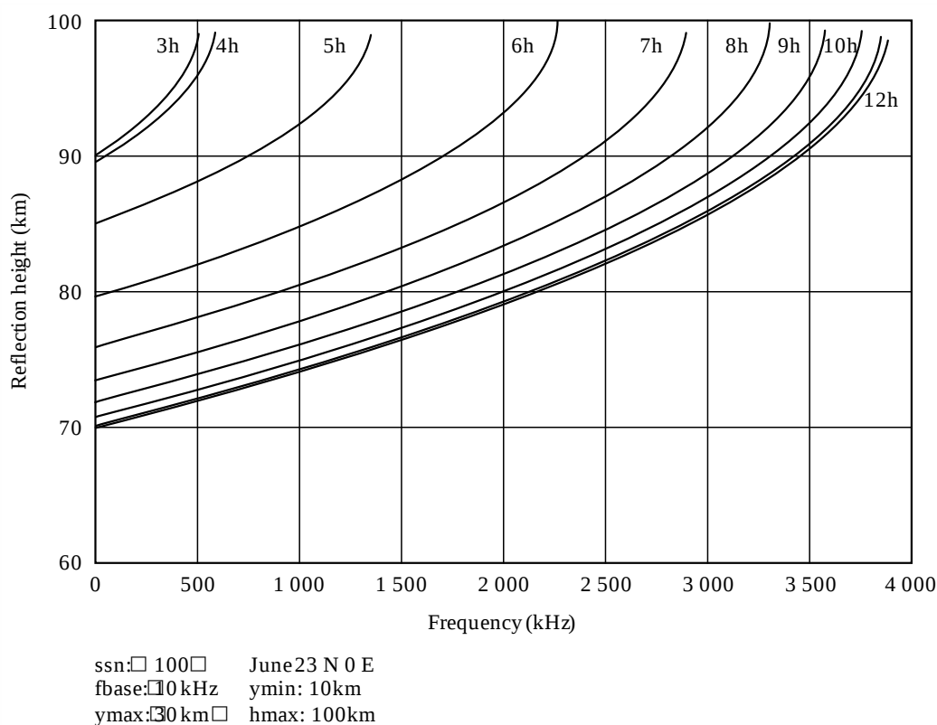
Variation in the height of reflection layer with local time
