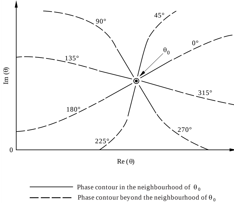
FIGURE 17 Phase contour behaviour near a zero of F(q)
