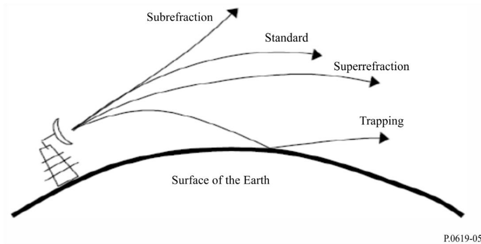
FIGURE 5 Tropospheric refraction
