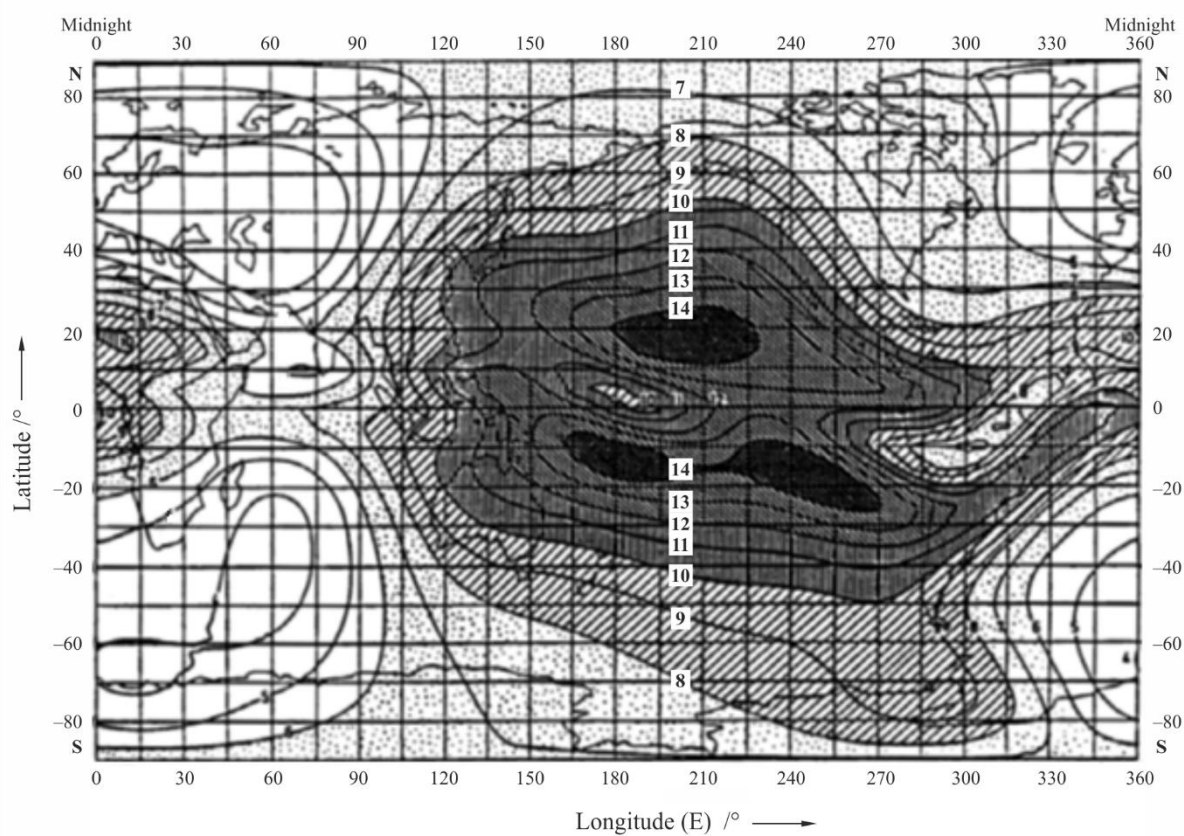
FIGURE 7 Ionospheric refraction
