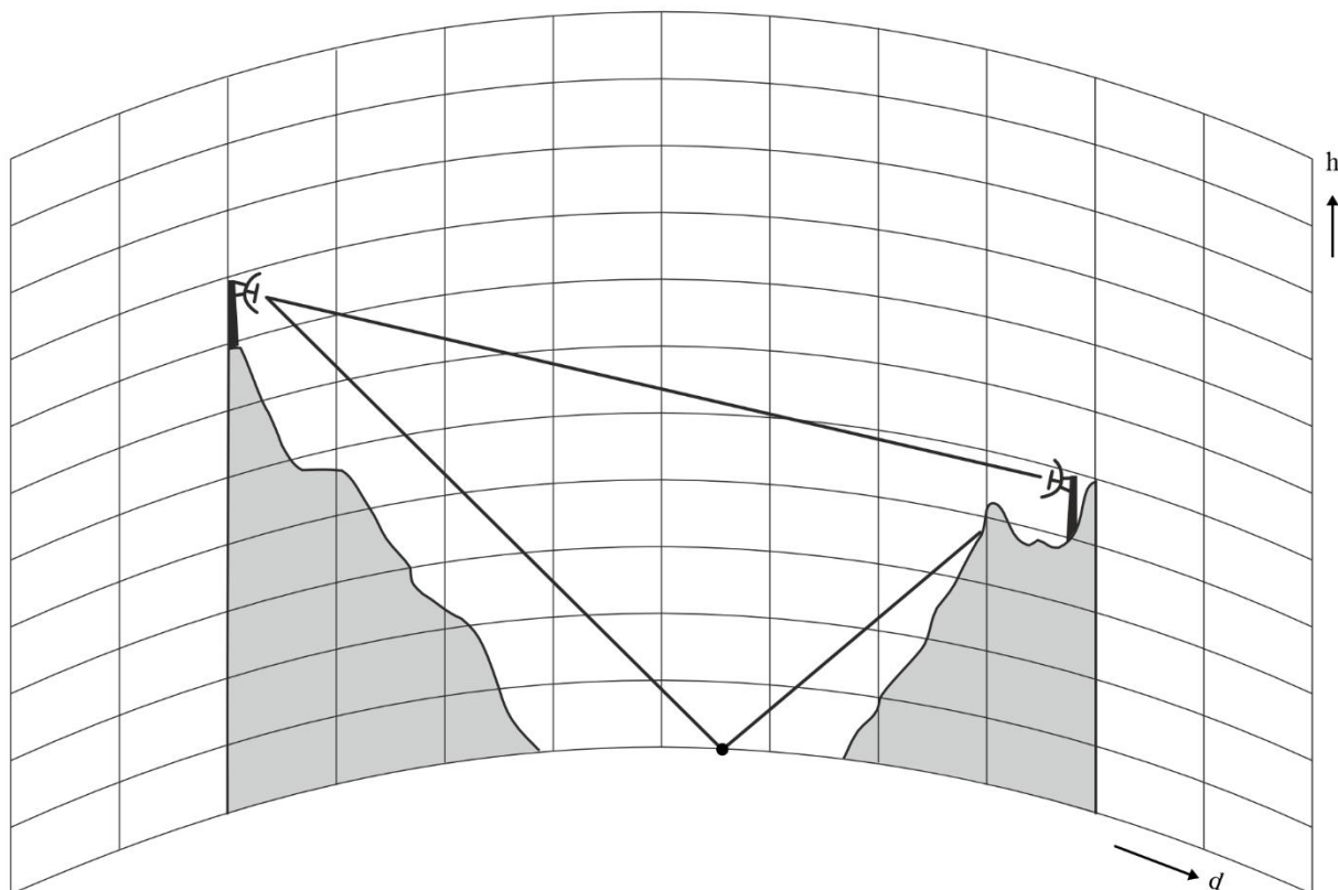
FIGURE 9 Example of shielding of antenna from specular reflection
