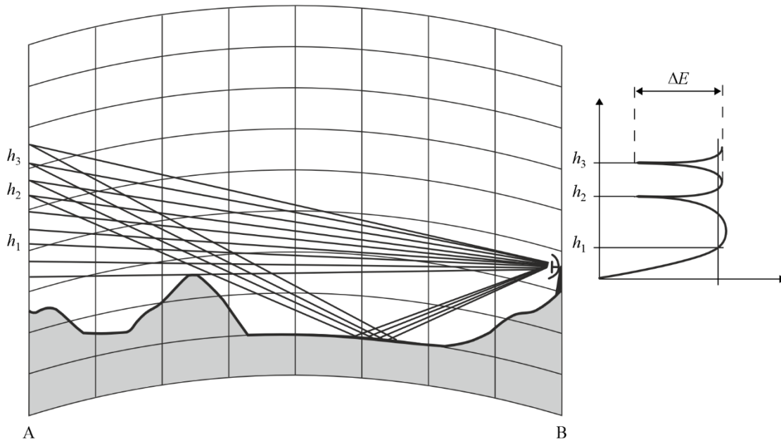
FIGURE 11 Measurement of \Delta E (dB) from height gain pattern
