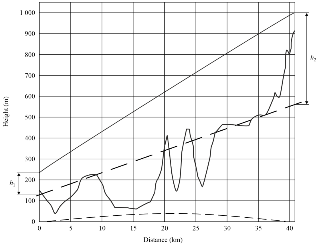
FIGURE 10 Path with reflective terrain
