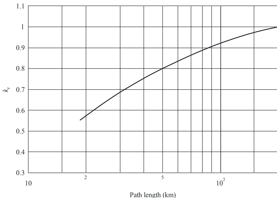
FIGURE 2 Value of k_e exceeded for approximately 99.99% of the time (continental temperate climate)
