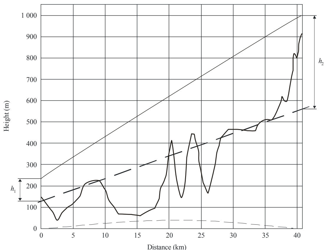
FIGURE 9 Path with reflective terrain
