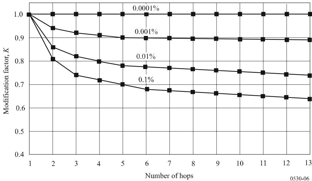
FIGURE 6 Modification factor for joint rain attenuation on a series of tandem hops of a approximately 4.6 km each for several exceedance probability levels for each link (May 1975-March 1979)
