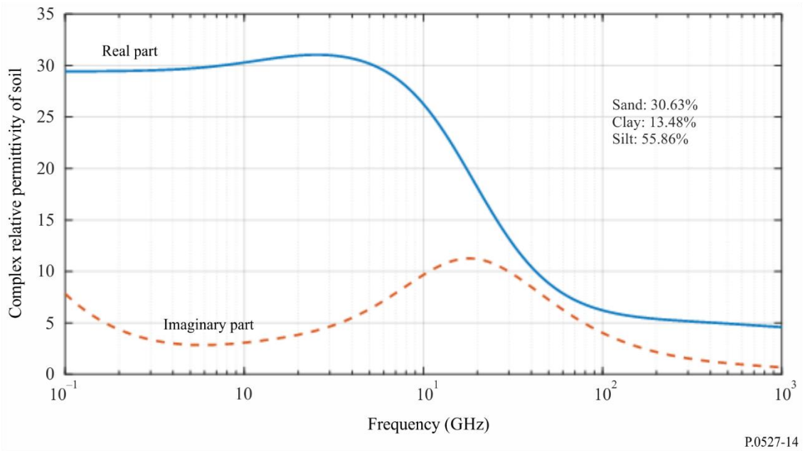
FIGURE 14 Complex relative permittivity of a silty loam soil as a function of frequency ( m_v = 0.5 , T = 23\text{ }^{\circ}\text{C} , \rho_s = 2.59 , \rho_b = 1.5750\text{ g cm}^{-3} )
