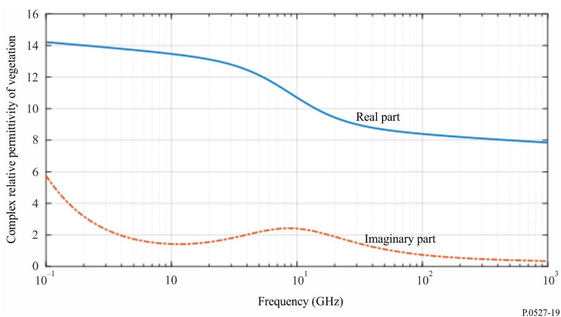
FIGURE 19 Complex relative permittivity of vegetation as a function of frequency ( M_g = 0.68, T = -7\text{ }^{\circ}\text{C} )
