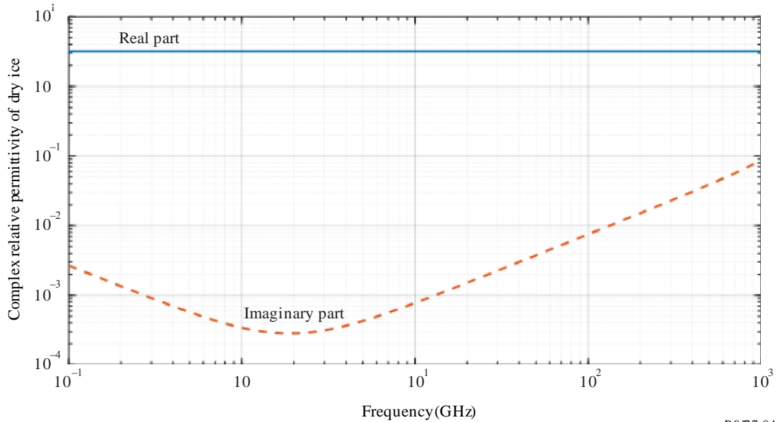
FIGURE 4 Complex relative permittivity of dry ice as a function of frequency ( T = -10\text{ }^{\circ}\text{C} )
