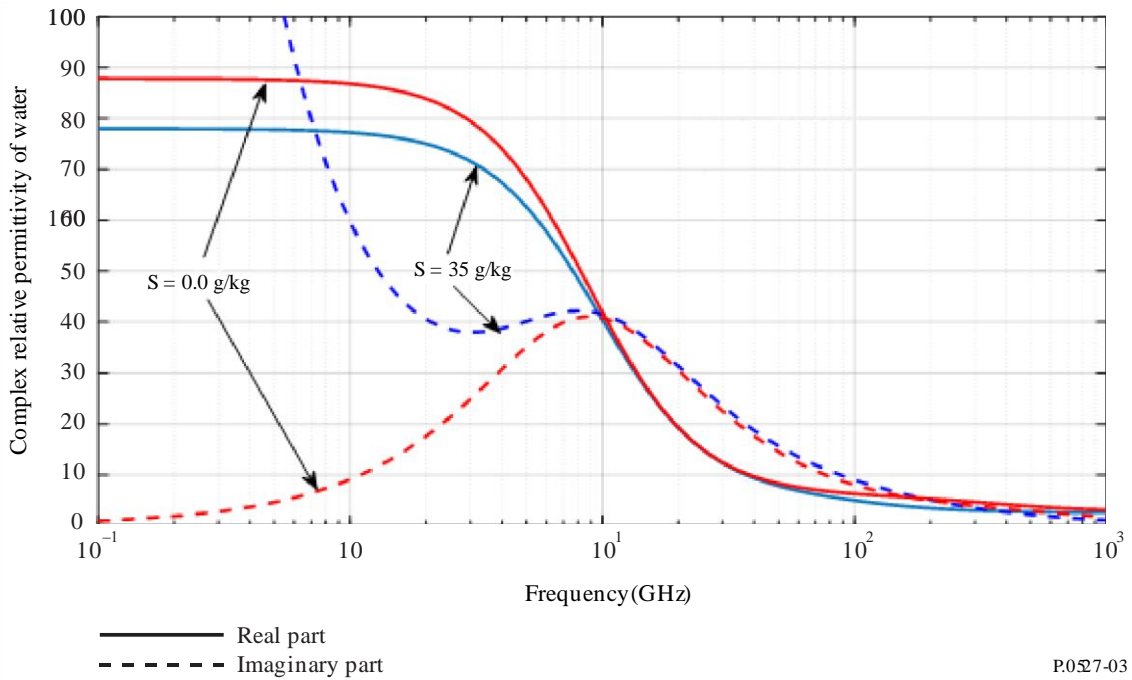
FIGURE 3 Complex relative permittivity of pure and sea water as a function of frequency ( T = 0\text{ }^{\circ}\text{C} )
