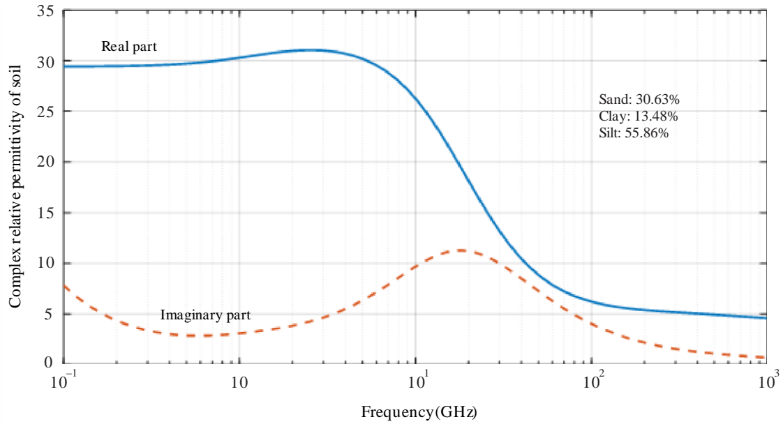
FIGURE 7 Complex relative permittivity of a silty loam soil as a function of frequency ( m_v = 0.5 , T = 23\text{ }^\circ\text{C} , \rho_s = 2.59 , \rho_b = 1.5750\text{ g cm}^{-3} )
