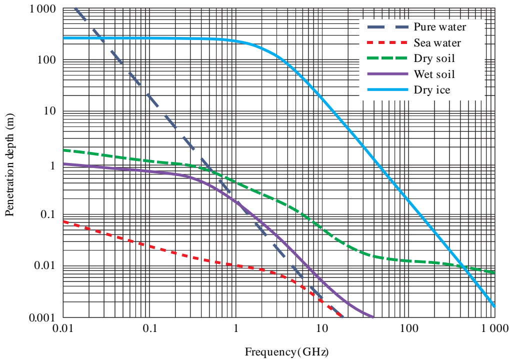
Penetration depth of surface types as a function of frequency
