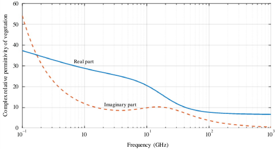
FIGURE 10 Complex relative permittivity of vegetation as a function of frequency ( M_g = 0.68, T = 22 \text{ }^\circ\text{C} )
