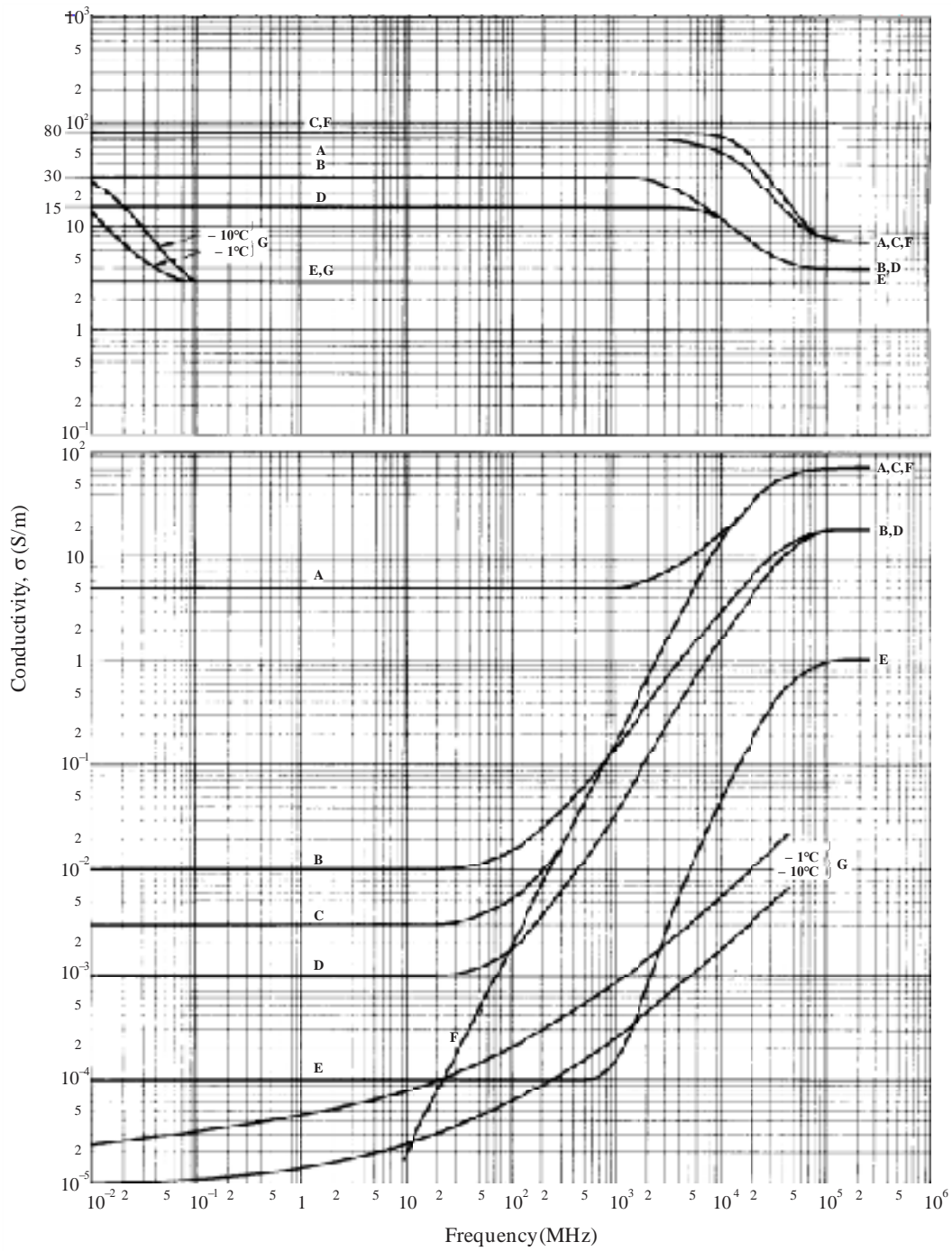
FIGURE 14 Relative permittivity \epsilon_r , and conductivity \sigma , as a function of frequency
