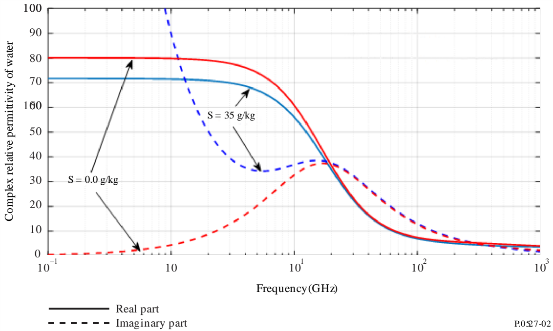
FIGURE 2 Complex relative permittivity of pure and sea water as a function of frequency ( T = 20\text{ }^{\circ}\text{C} )
