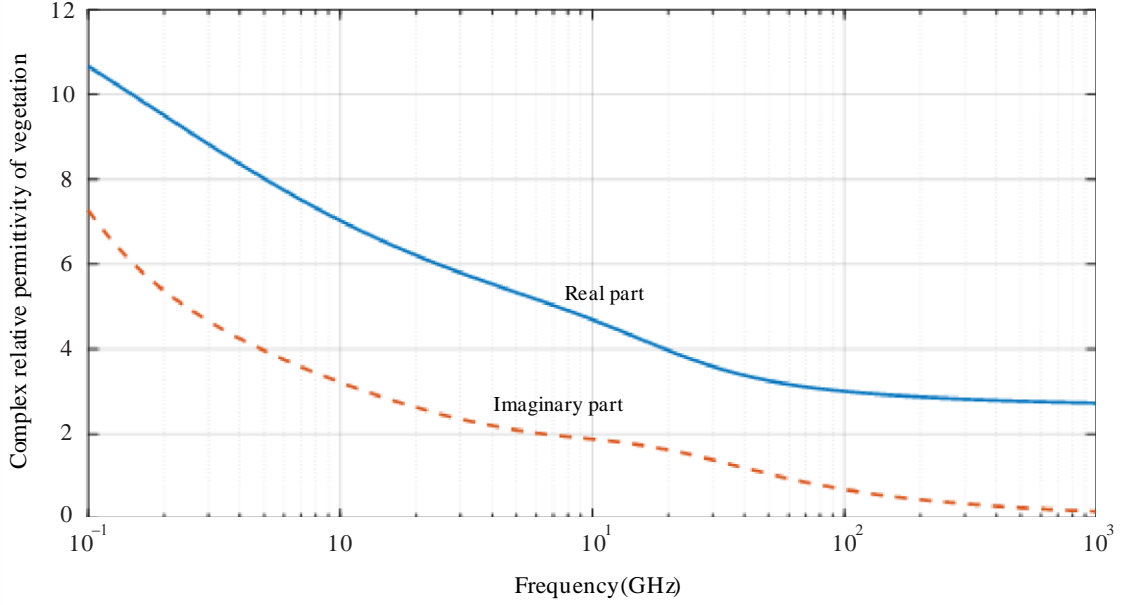
FIGURE 11 Complex relative permittivity of vegetation as a function of frequency ( M_g = 0.26, T = 22 \text{ }^\circ\text{C} )
