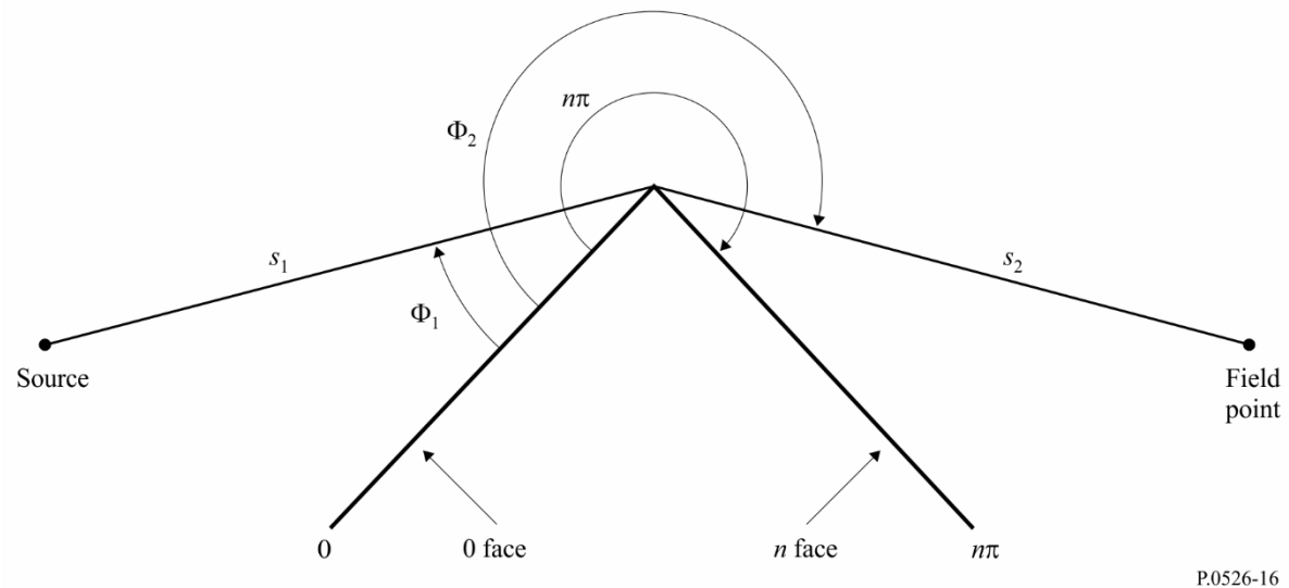
FIGURE 16 Geometry for application of UTD wedge diffraction
