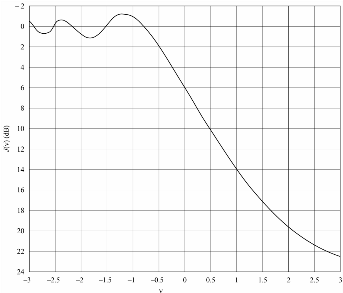
Knife-edge diffraction loss
