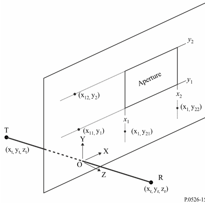
FIGURE 15 Geometry for a single rectangular aperture
