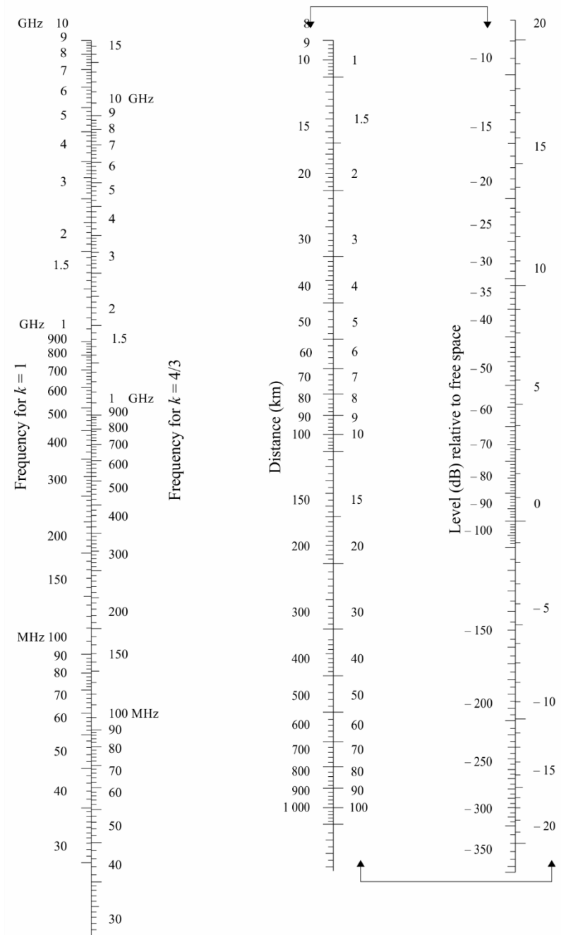
FIGURE 5 Diffraction by a spherical Earth – effect of distance
