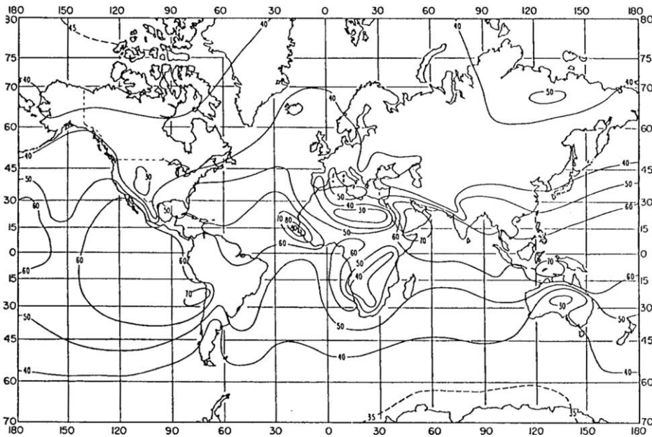
Monthly mean values of \Delta N : November
