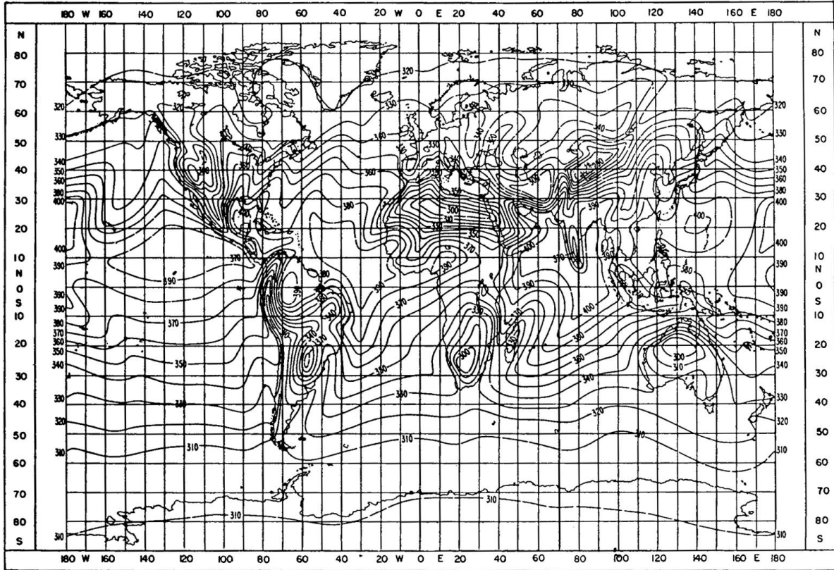
FIGURE 2 Monthly mean values of N_0 : August
