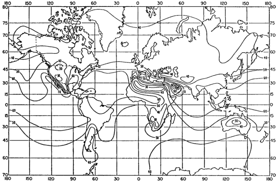
Monthly mean values of \Delta N : August
