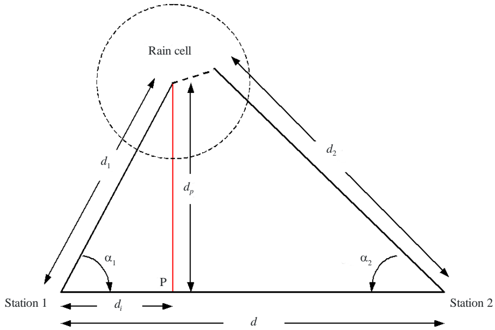
FIGURE 6 Plan view of geometry for side scattering
