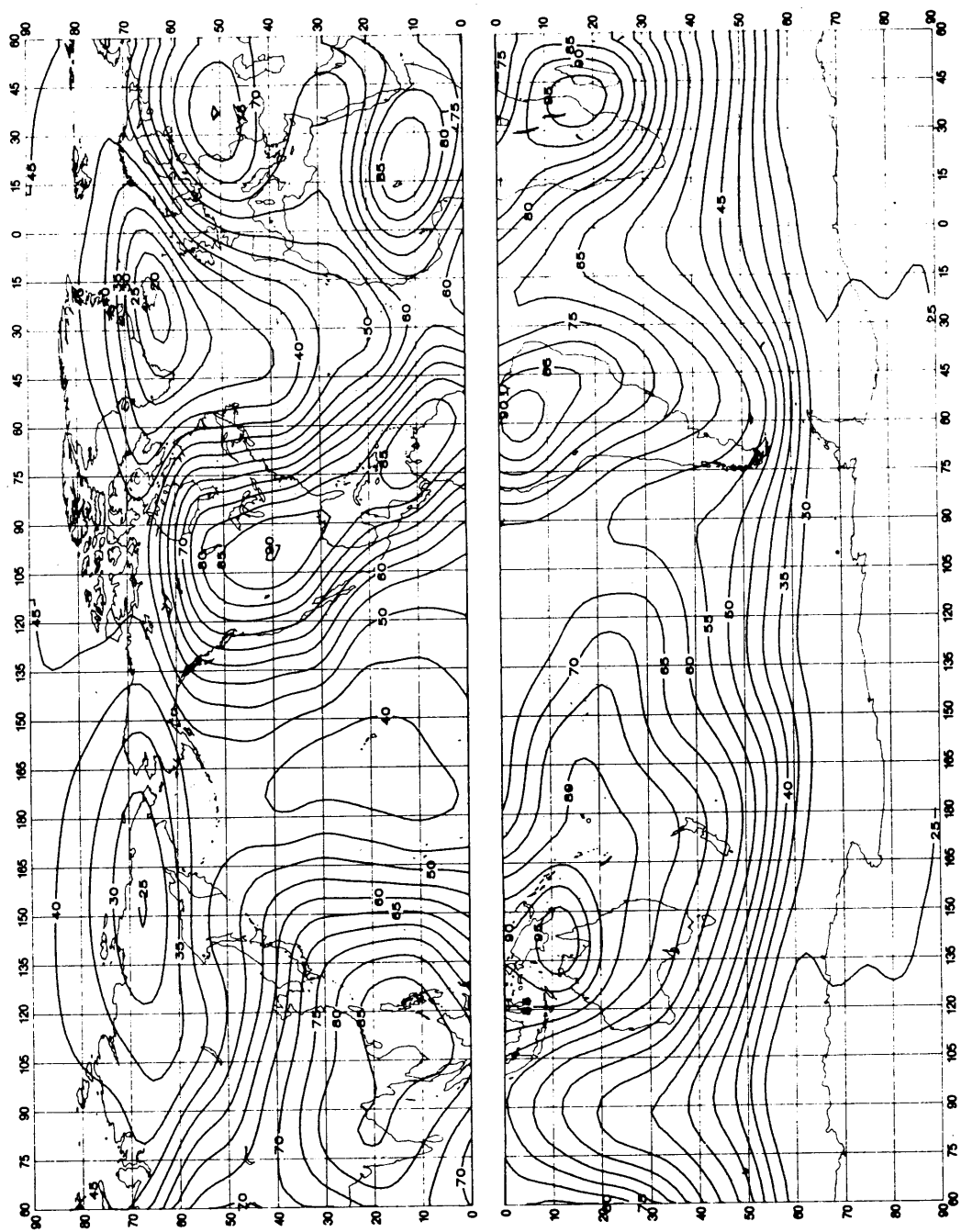
图31a-大气无线电噪声的预计值, F_{am} (1 MHz的dB高于 kT_{0b} ) (夏季; 1600-2000LT)
