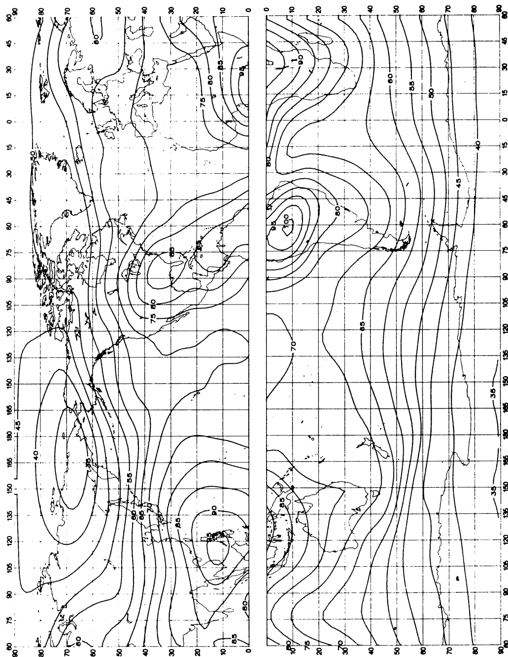
图21a-大气无线电噪声的预计值, F_{am} (1 MHz的dB高于 kT_0b ) (春季; 0000-0400LT)
