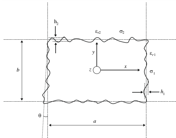
FIGURE 8 Cross-section of waveguide and material constants
