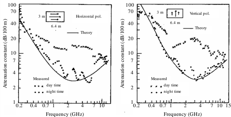
Attenuation constant comparison for day and night
