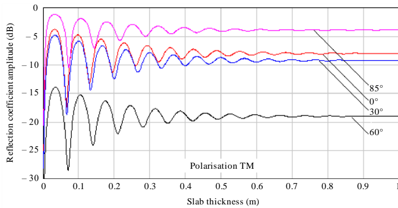
Reflection coefficient for a concrete slab at 1 GHz, TM polarisation
