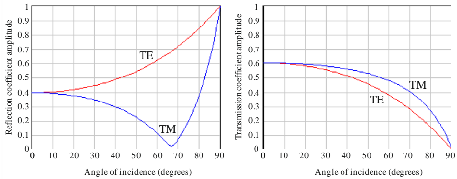
FIGURE 2 Reflection and transmission coefficients for air/concrete interface at 1 GHz
