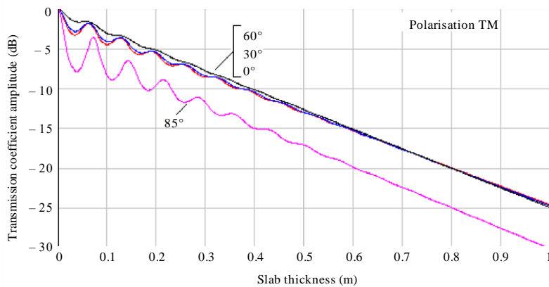
Transmission coefficient for a concrete slab at 1 GHz, TM polarisation
