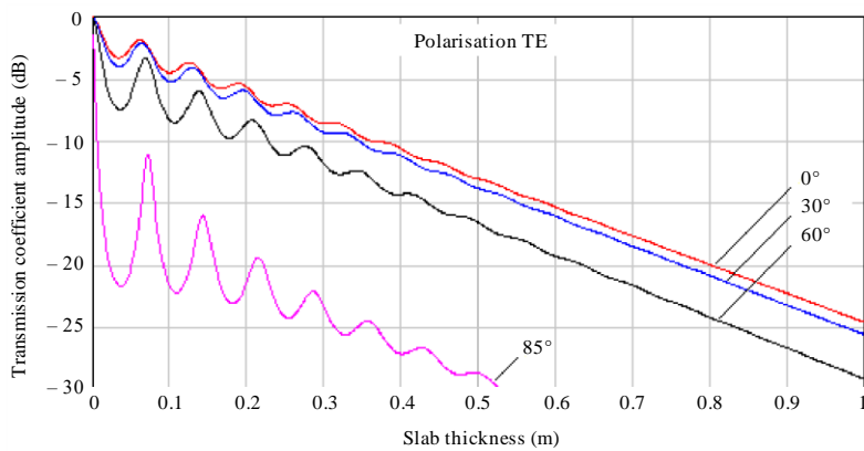
Transmission coefficient for a concrete slab at 1 GHz, TE polarisation
