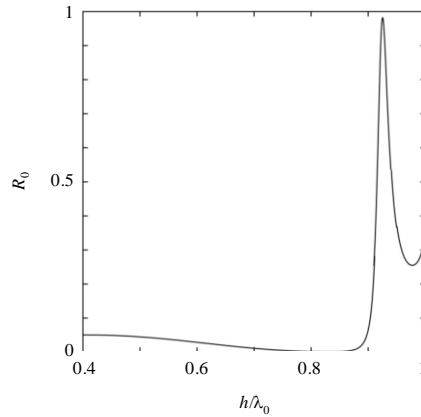
FIGURE 12 Power reflection coefficient R_0 as functions of the normalized wavelength h/\lambda_0 at normal incidence electric field E_z^{in}
