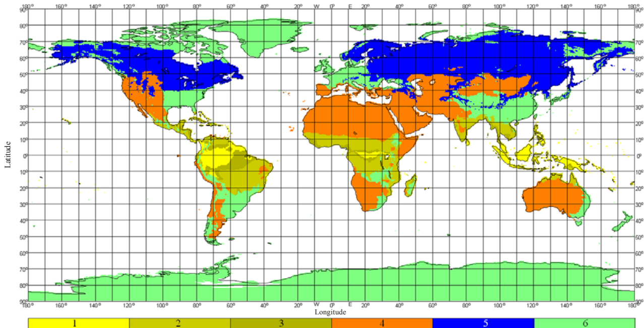
FIGURE E.1 Climatic zones
