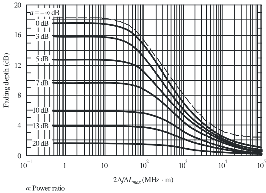
FIGURE 12 Relationship between fading depth and 2\Delta f\Delta L_{max}
