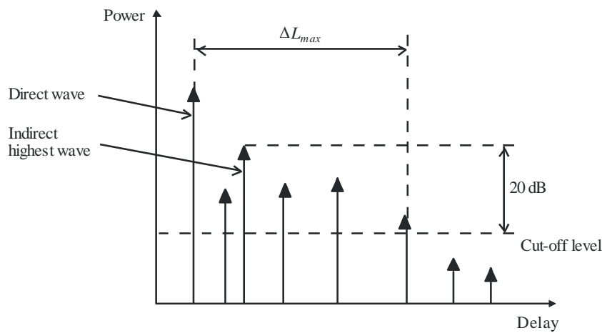
FIGURE 13 Model for calculating \Delta L_{max}
