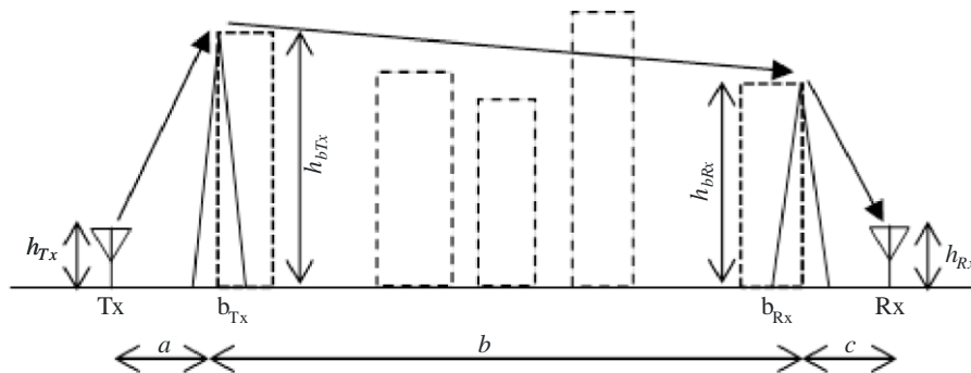
FIGURE 11 Side view of building geometry and parameters
