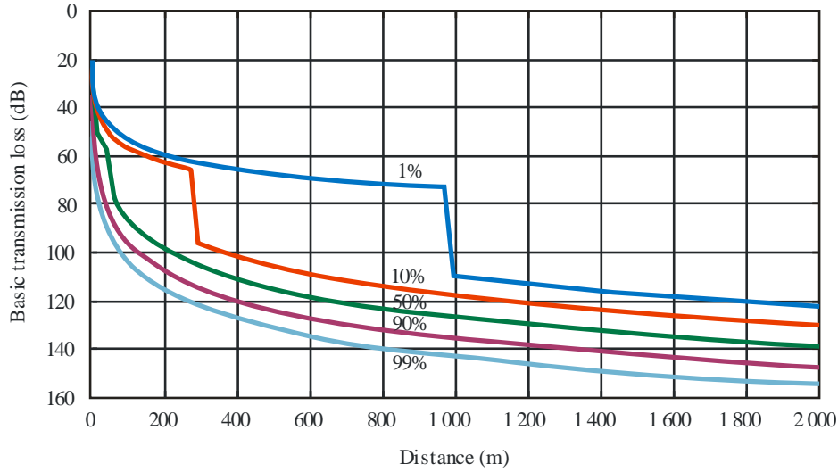
FIGURE 5 Curves of basic transmission loss not exceeded for 1, 10, 50, 90 and 99% of locations (frequency = 400 MHz, suburban)
