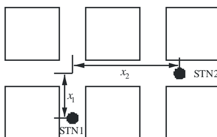
FIGURE 6 1-Turn NLoS Link between Station 1 and Station 2
