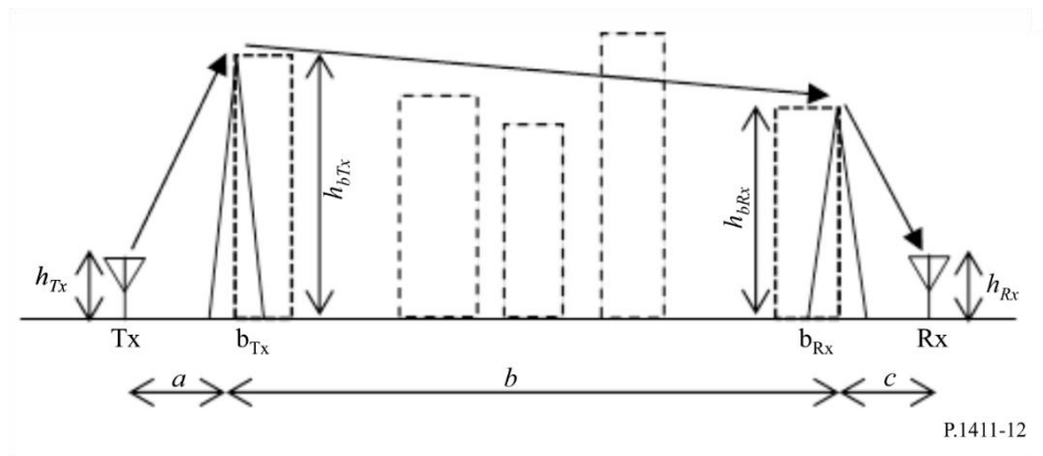
FIGURE 12 Side view of building geometry and parameters
