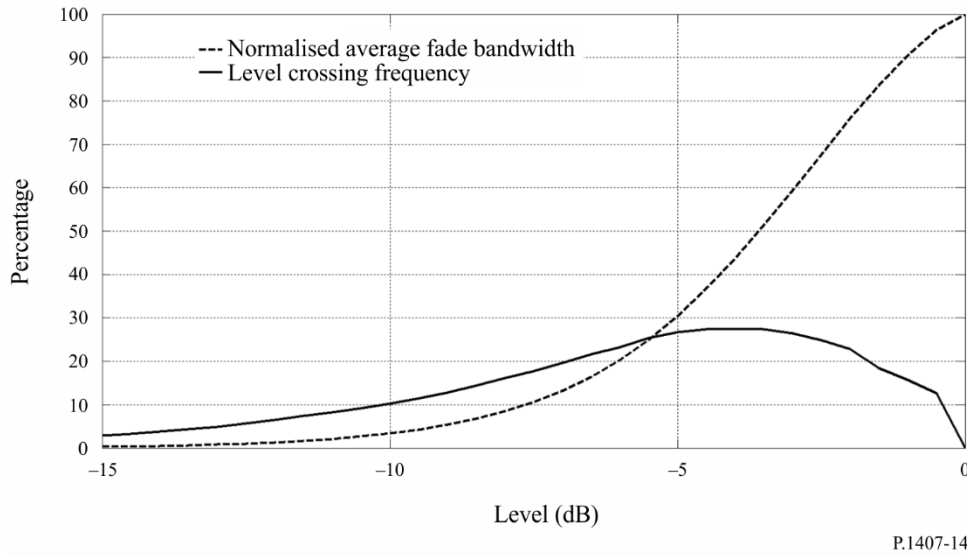
Normalized average fade bandwidth and level crossing frequency
