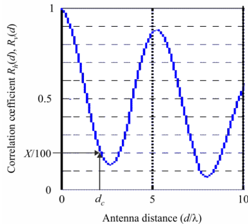
FIGURE 9 Spatial correlation distance
