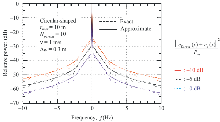
FIGURE 8 Power spectrum in circular room
