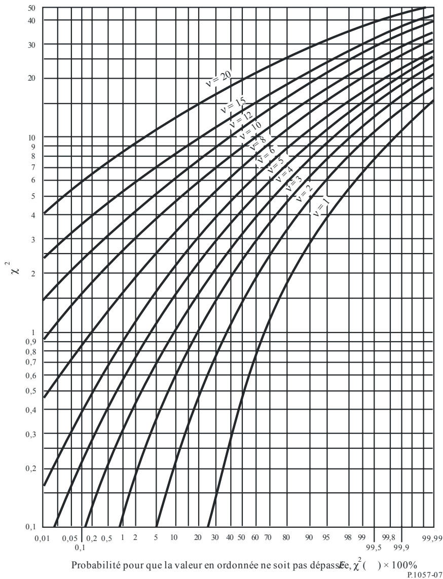
FIGURE 7 \chi^2 distribution
