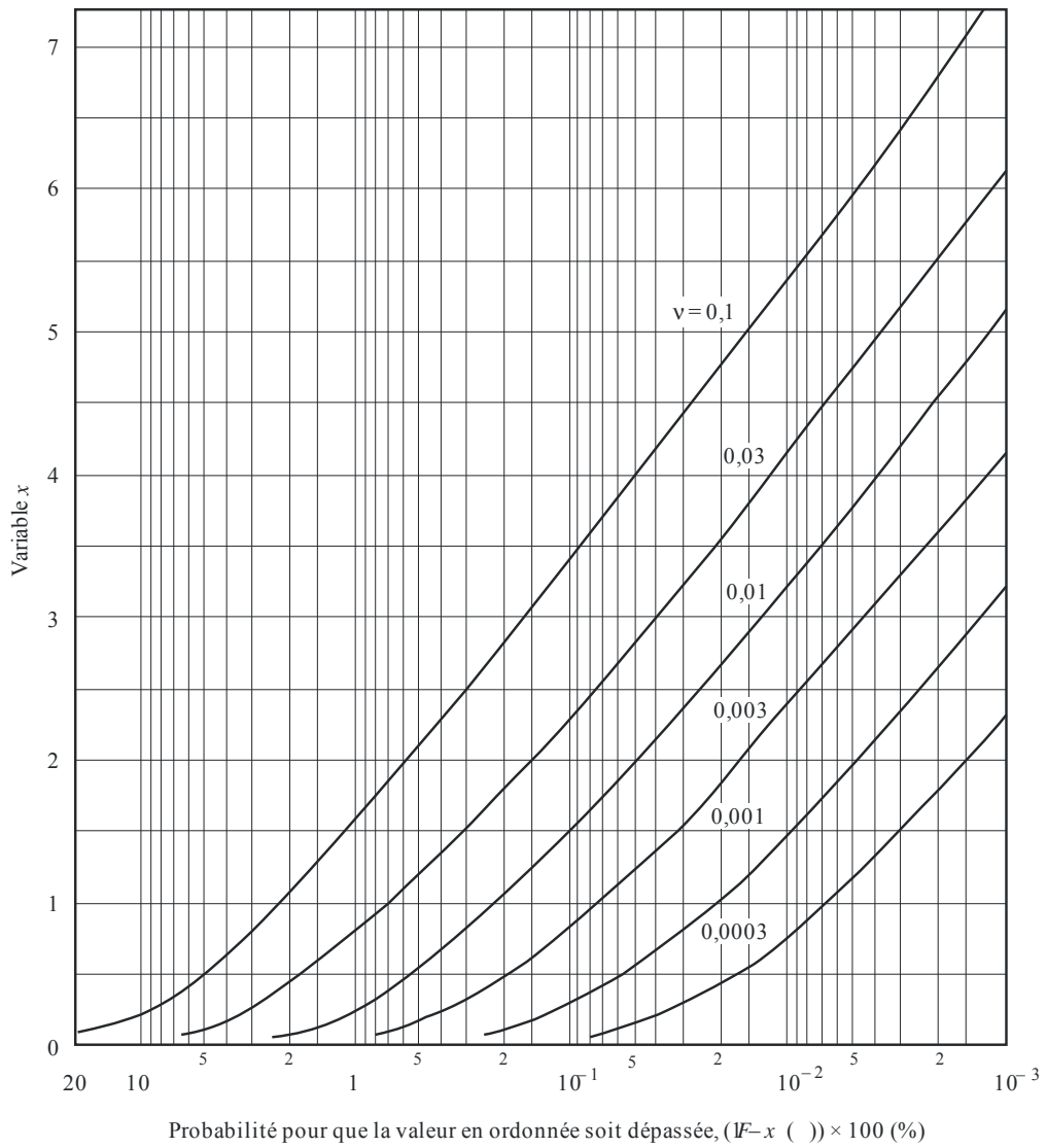
FIGURE 5 Distribution gamma ( \alpha = 1, \nu \leq 0,1 )
