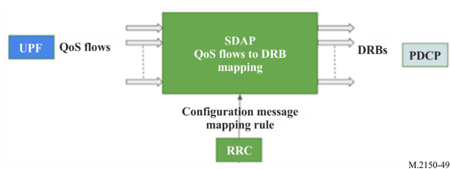
FIGURE 49 SDAP downlink architecture
