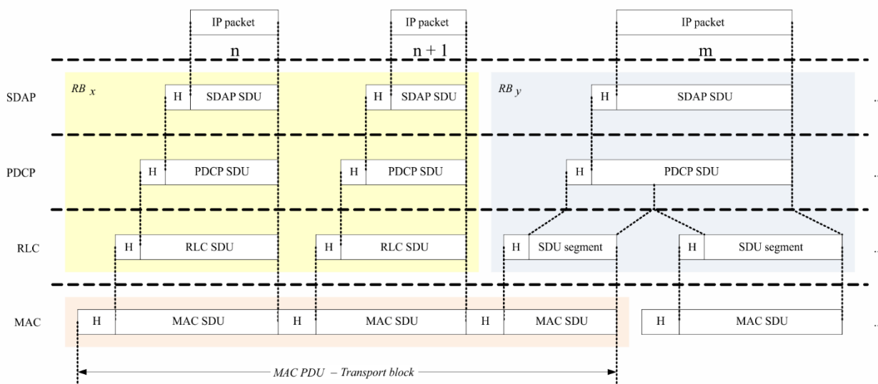
FIGURE 74 Data flow example
