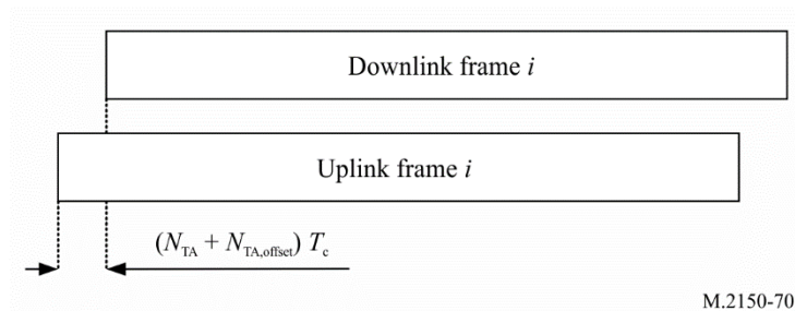
FIGURE 70 Uplink-downlink timing relation
