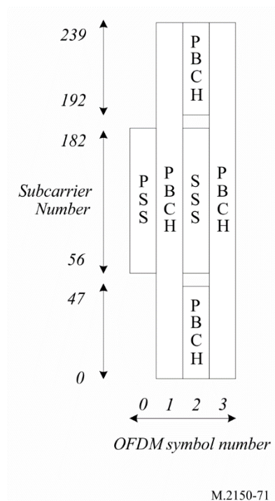
FIGURE 71 Time-frequency structure of SSB
