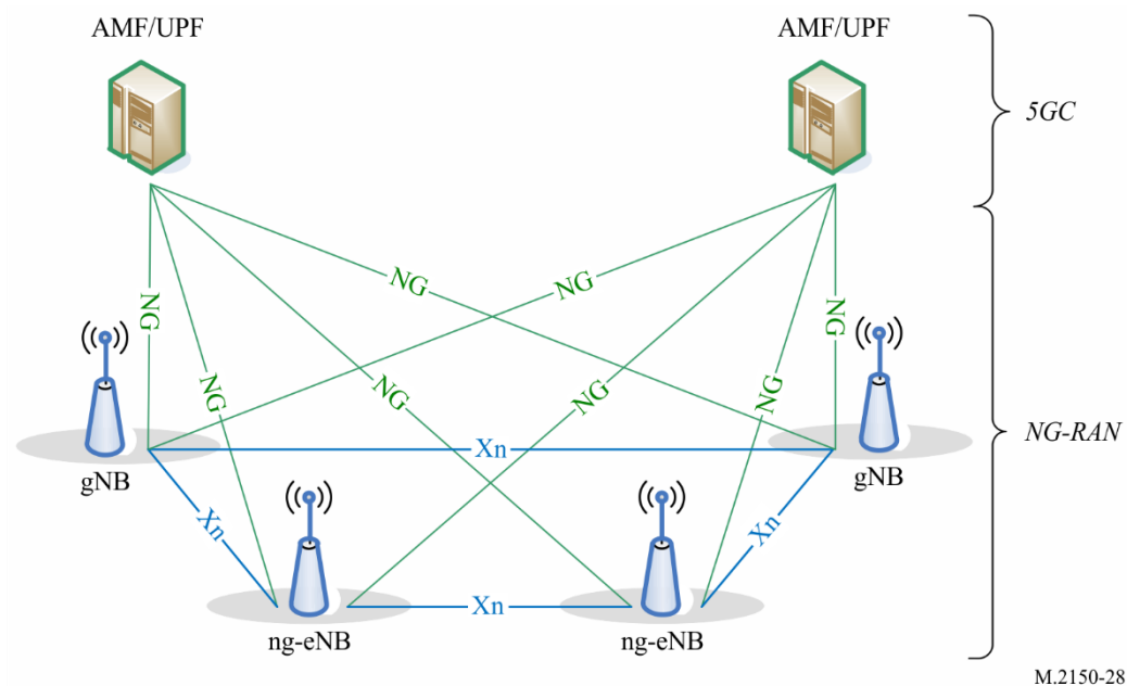
FIGURE 28 Overall Architecture
