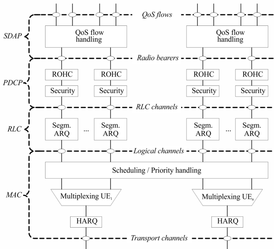
FIGURE 72 Downlink layer 2 structure
