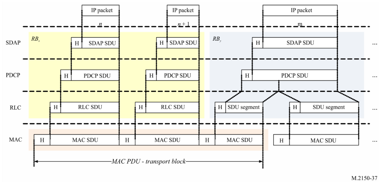
FIGURE 37 Data flow example
