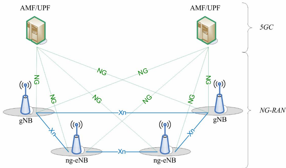
FIGURE 65 Overall architecture
