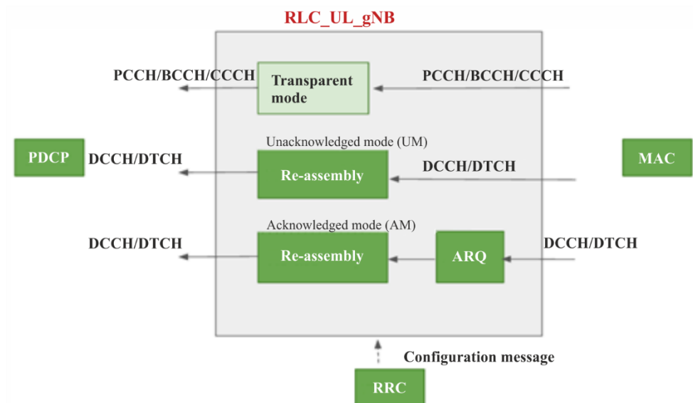
Uplink architecture of RLC
