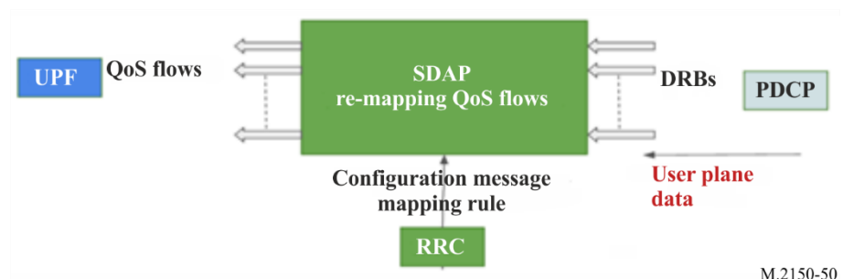
FIGURE 50 SDAP uplink architecture
