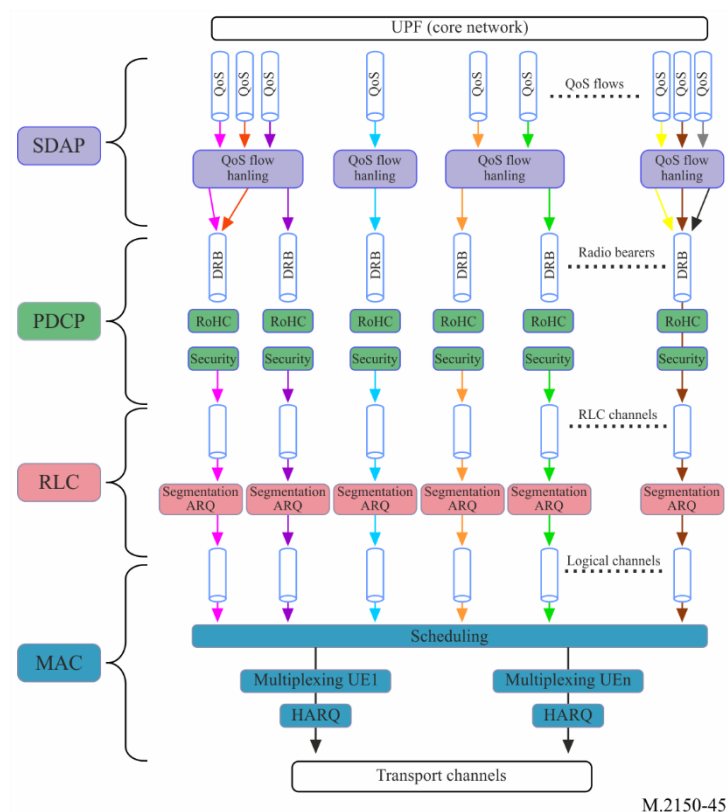
FIGURE 45 Downlink user plane architecture of Layer 2
