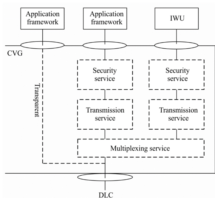
FIGURE 64 CVG architecture
