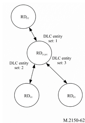
FIGURE 62 DLC entity sets for RD operating in both FT and PT mode
