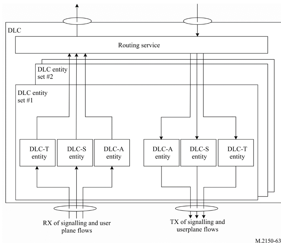
FIGURE 63 DLC architecture
