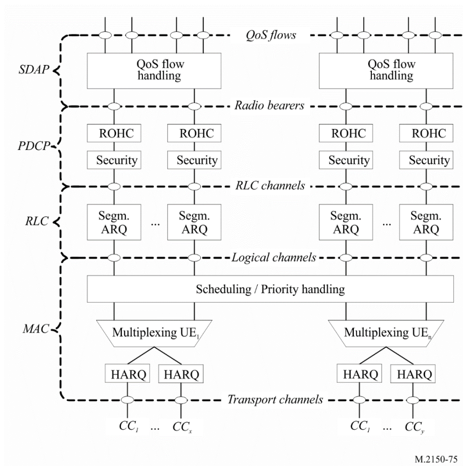
FIGURE 75 Layer 2 structure for DL with CA configured
