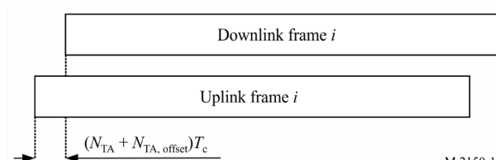
Uplink-downlink timing relation
