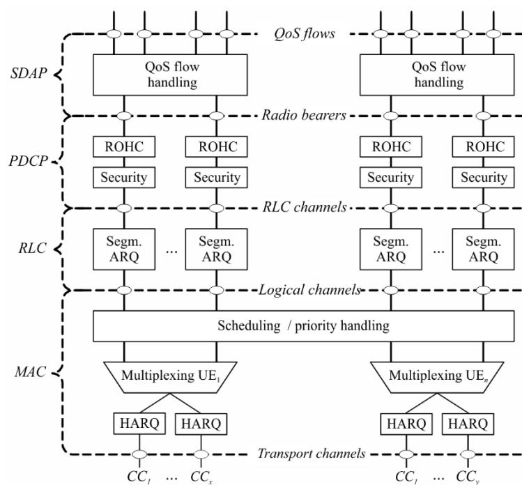
FIGURE 24 Layer 2 structure for DL with CA configured
