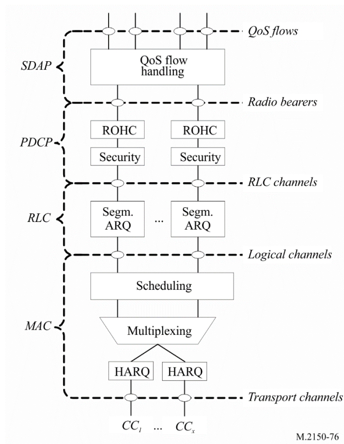
FIGURE 76 Layer 2 structure for UL with CA configured
