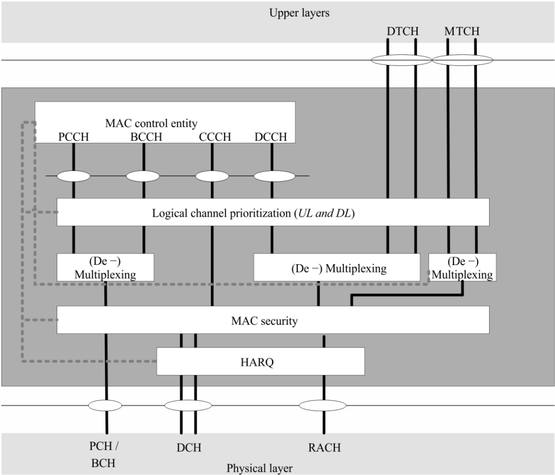
FIGURE 60 MAC structure overview
