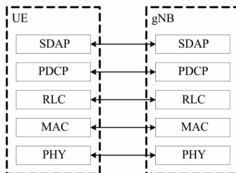
FIGURE 66 User Plane protocol stack
