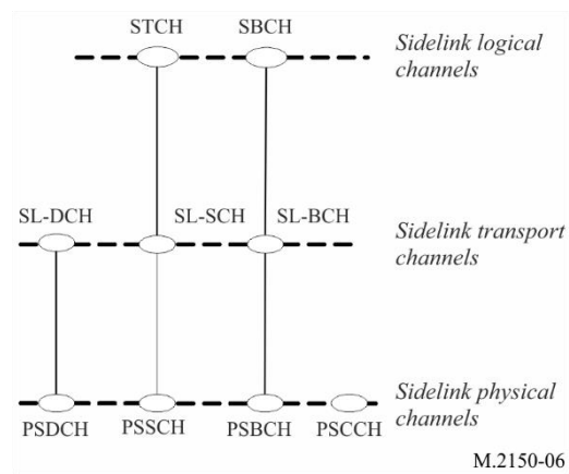
FIGURE 6 Sideline channel mapping
