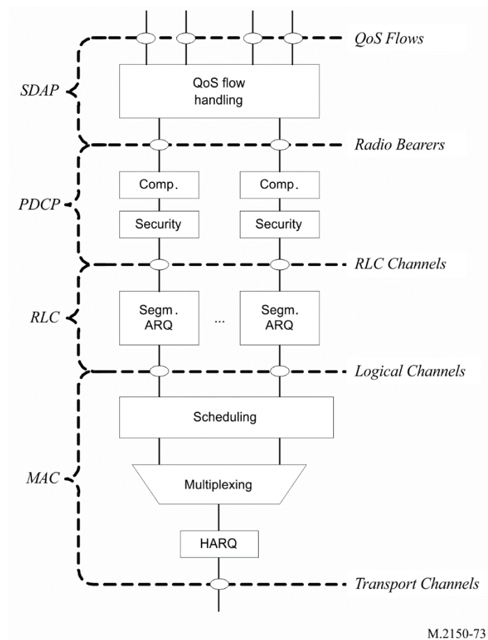
FIGURE 73 Uplink layer 2 structure
