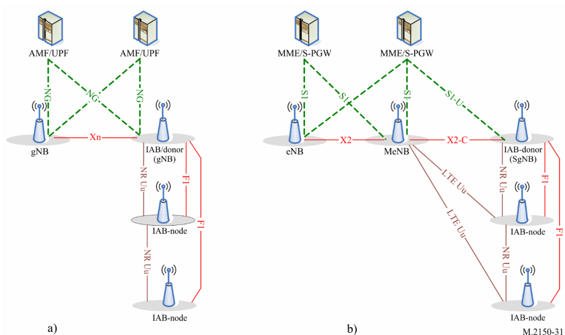
FIGURE 31 IAB architecture; a) IAB-node using SA mode with 5GCN; b) IAB-node using EN-DC
