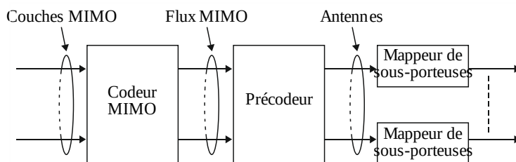
FIGURE 19 Structure MIMO
