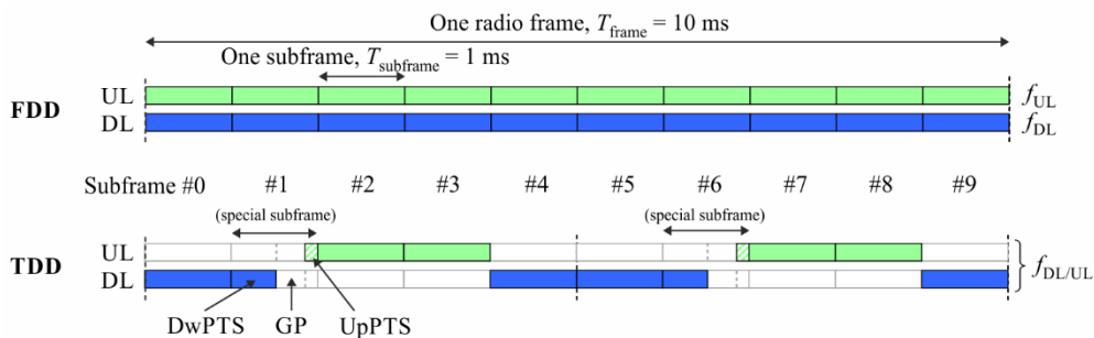
FIGURE 11 Uplink/downlink time/frequency structure in case of FDD and TDD
