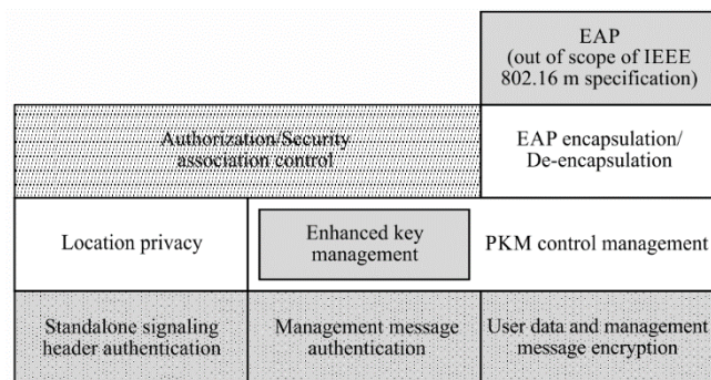
FIGURE 23 Functional blocks of security architecture
