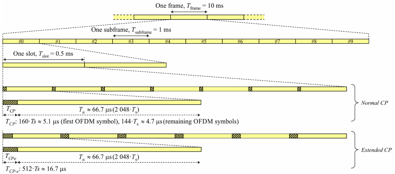
FIGURE 10 LTE-Advanced time-domain structure
