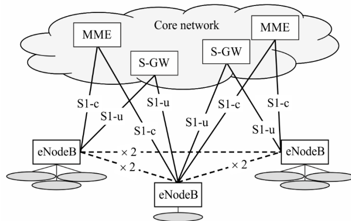
FIGURE 1 Radio-access network interfaces
