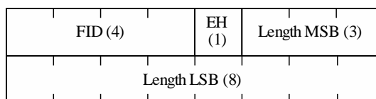
FIGURE 2.9 Advanced generic MAC headers
