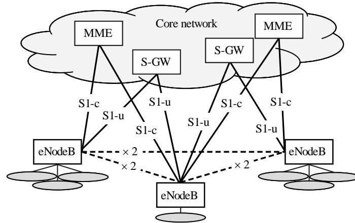
FIGURE 1.1 Radio-access network interfaces
