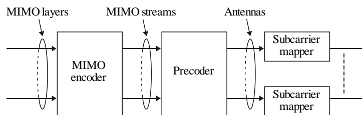
MIMO structure
