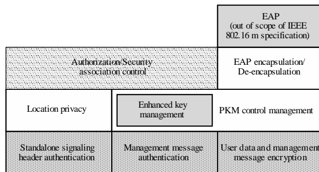
FIGURE 2.11 Functional blocks of security architecture
