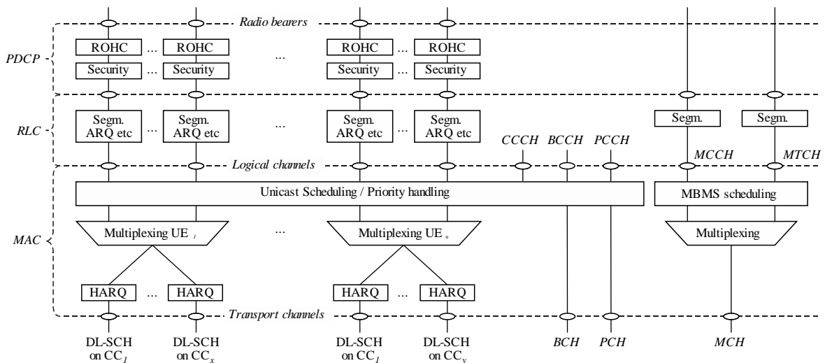
FIGURE 1.2 Downlink L2 protocol structure
