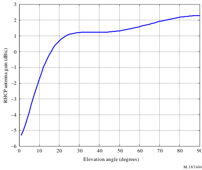
FIGURE 4 Example receive antenna gain as a function of elevation angle
