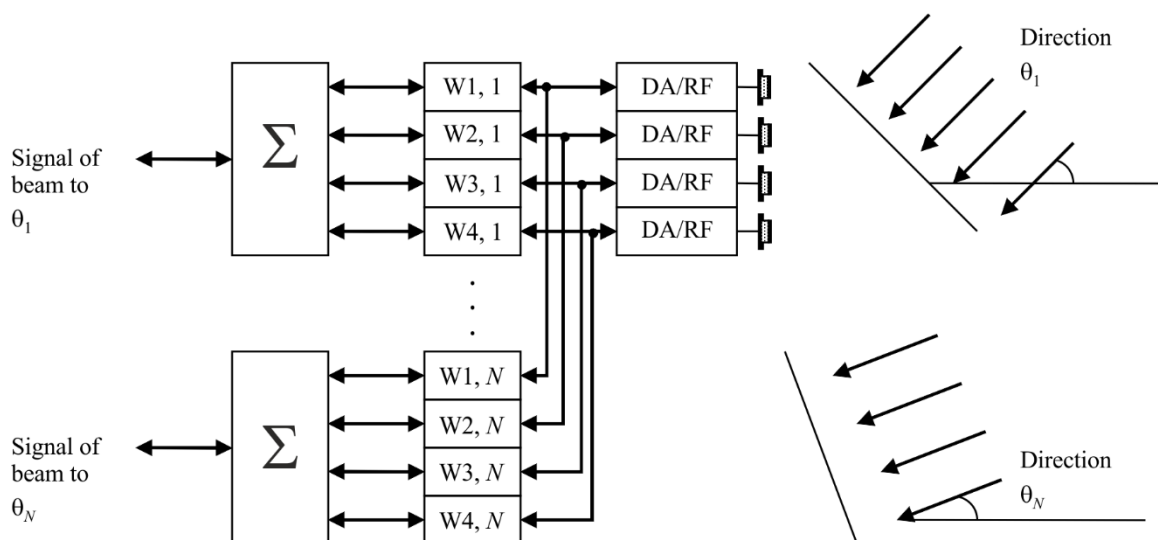
FIGURE 1 Multiple beam antenna
