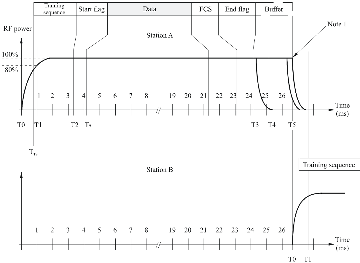
FIGURE 6 Transmission timing
