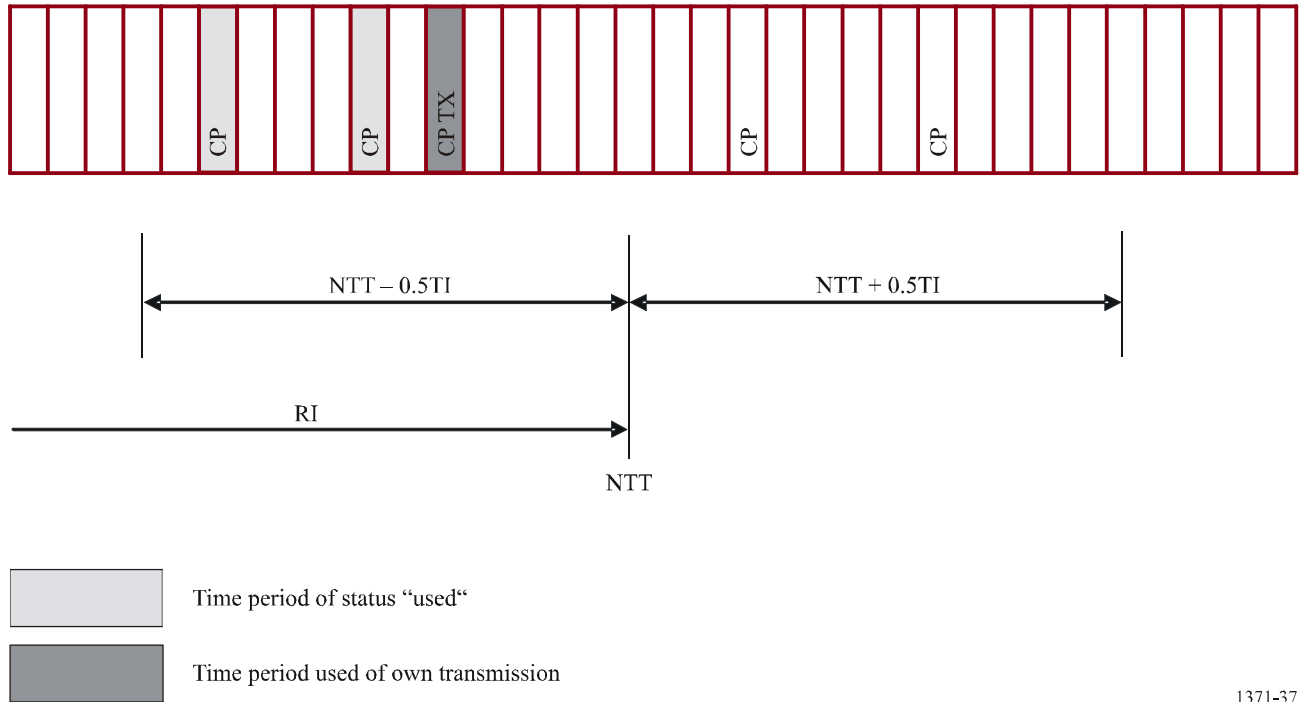
FIGURE 37 Example of CS-TDMA access
