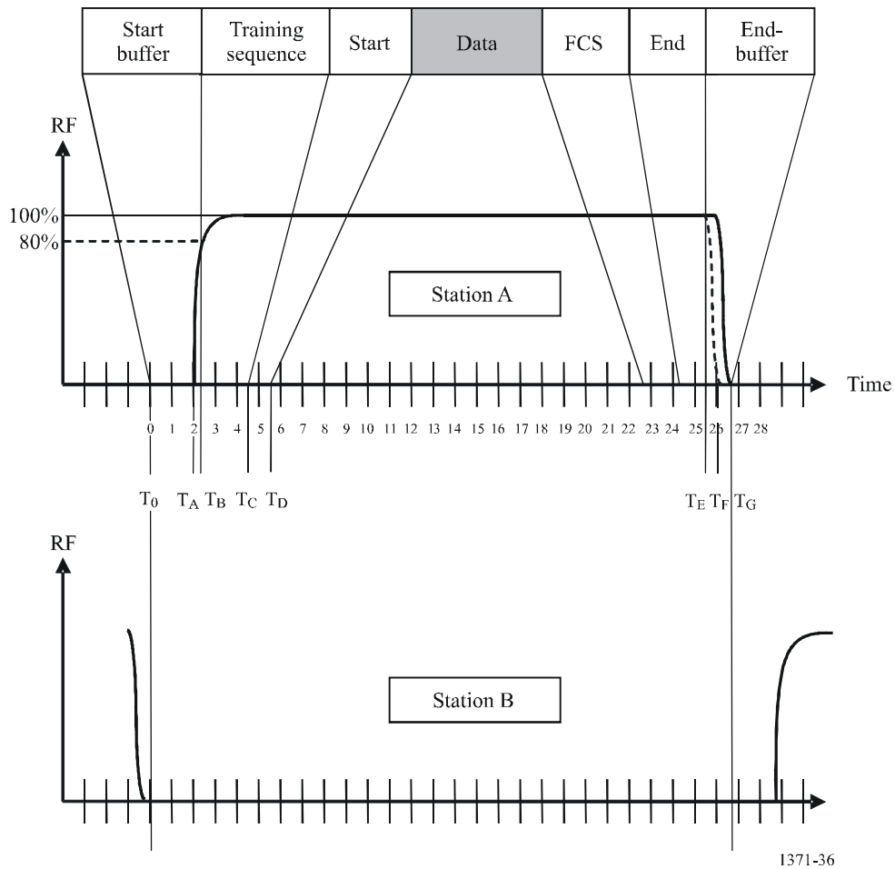
FIGURE 36 Transmission timing
