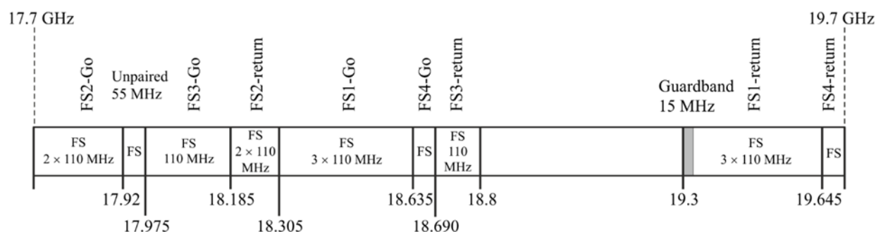
FIGURE 11 Channelization plan for the 17.7-19.7 GHz band of Annex 6
