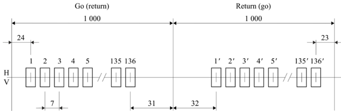
FIGURE 6 Radio-frequency channel arrangement for low capacity fixed wireless systems with 7 MHz channel spacing operating in the 18 GHz band (United Kingdom) (All frequencies in MHz)
