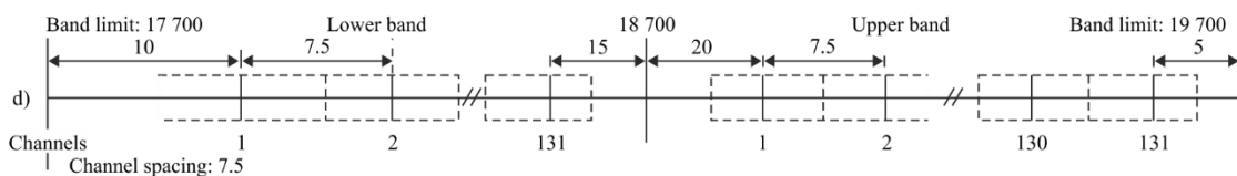
FIGURE 9 Radio-frequency channel arrangement for low capacity fixed wireless system with 7.5 MHz spacing in co-channel arrangement
