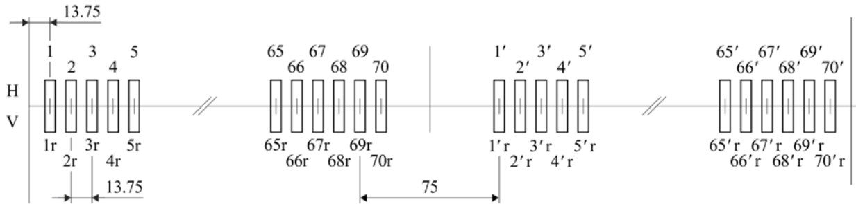
FIGURE 7 Radio-frequency channel arrangement for medium capacity fixed wireless systems with 13.75 MHz channel spacing in co-channel arrangement (All frequencies in MHz)
