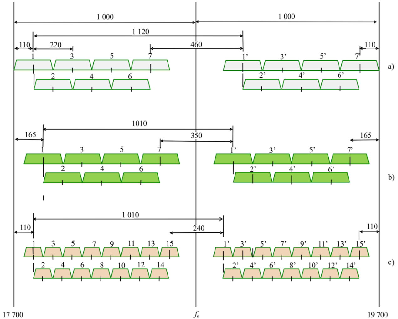
FIGURE 2 Radio-frequency channel arrangement for fixed wireless systems operating in the 17.7 to 19.7 GHz band (Interleaved arrangement) (All frequencies in MHz)
