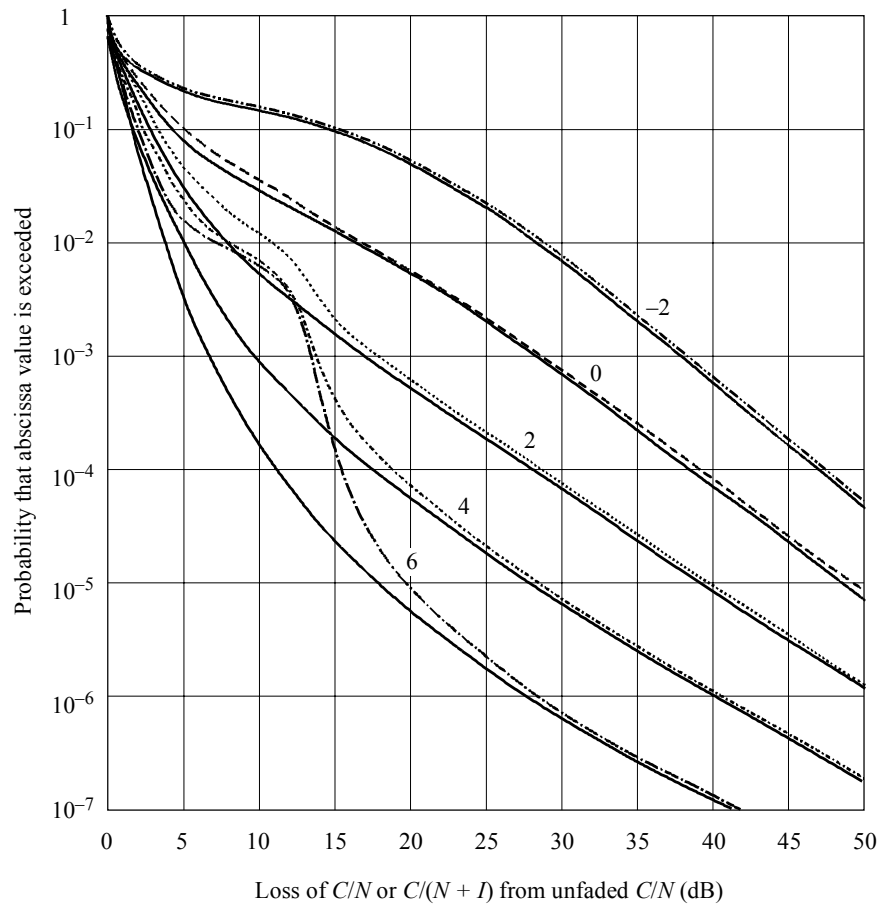
FIGURE 18 Cumulative probability distributions of the loss C/N and C/(N+I) from unfaded C/N from a simulation of a LEO-F constellation for non-diversity operation for a FS receiving antenna at 50^\circ azimuth from North with several values of parameter qt
