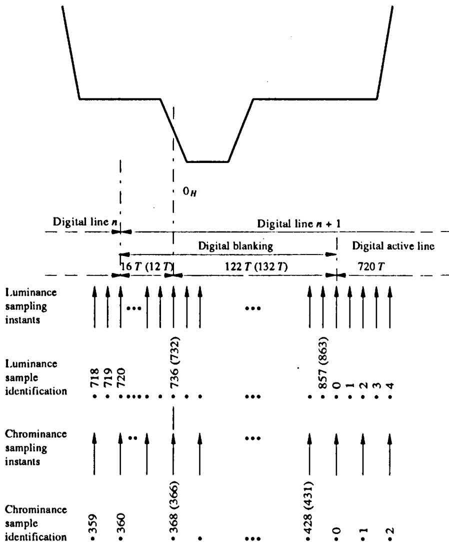
FIGURE 1 Relationship between video samples and the analogue line synchronization
